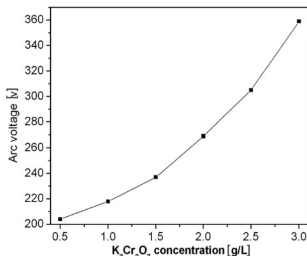
Figure 6. Relationship between the K_2Cr_2O_7 dose and the arcing voltage
