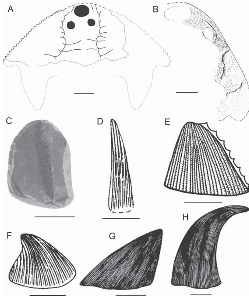
Text-fig. 2. Fossil fishes from the Silurian of north-western Hunan. A – reconstruction of Dayongaspis hunanensis Pan and Zeng, 1985. B – reconstruction of Konoceraspis grandoculus Pan, 1992. C – Shimenolepis graniferus Wang J.-Q., 1991, an incomplete left posterior plate (internal mould), ventral view. D – reconstruction of Sinacanthus wuchangensis P'an, 1959 (based on Zeng 1988 and Zhu 1998). E – reconstruction of Neosinacanthus planispinatus P'an and Liu in P'an et al. , 1975 (based on Zeng 1988 and Zhu 1998). F – reconstruction of Tarimacanthus bachuensis Zhu, 1998 (based on Zeng 1988). G – reconstruction of Eosinacanthus shanmenensis Liu, 1997. H – reconstruction of Hunanacanthus lixianensis Liu, 1997. Scale bars = 10 mm
