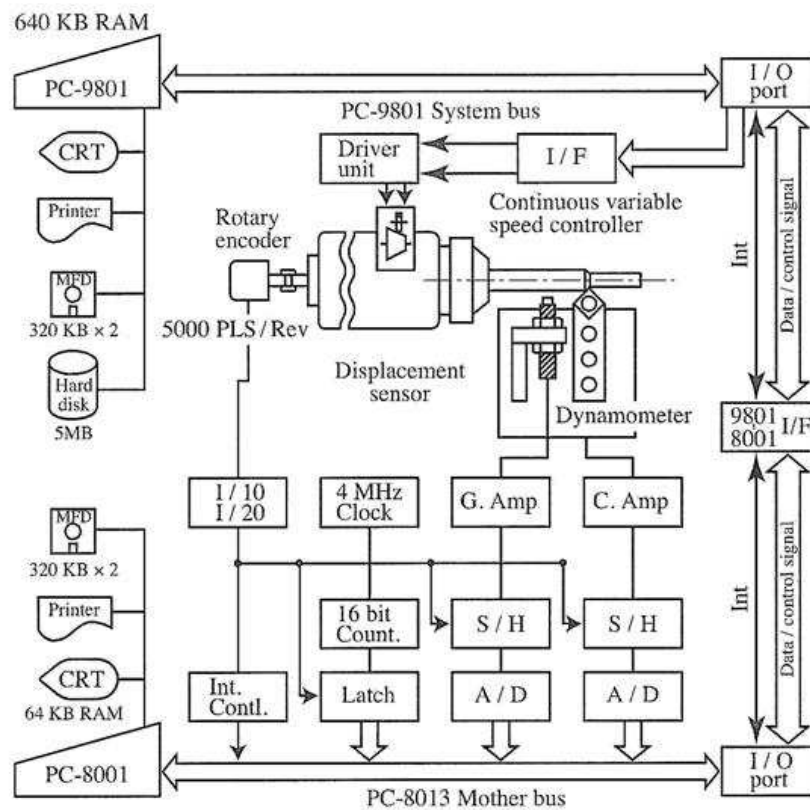
Fig. 25. Flow diagram of measurement system for analyzing phase relationship during chatter occurrence
