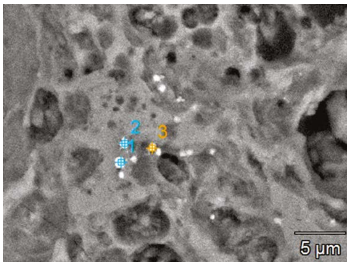
Fig. 2. SEM image of pyrrhotite grains in highly porous glass in fly ash from Bełchatów Power Station
