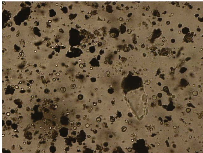
Fig. 1. Microscopic image of glass grains, quartz and unburned coal in fly ash from Bełchatów Power Station, transmitted light, one nicol, 400× magnification
