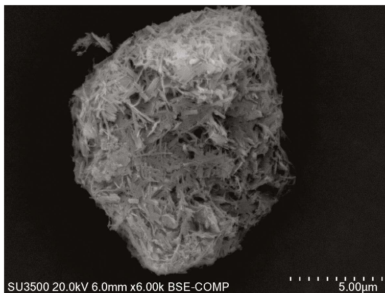
Fig. 7. SEM image of tobermorite rods and pitiglianoite bars, 6000× magnification
