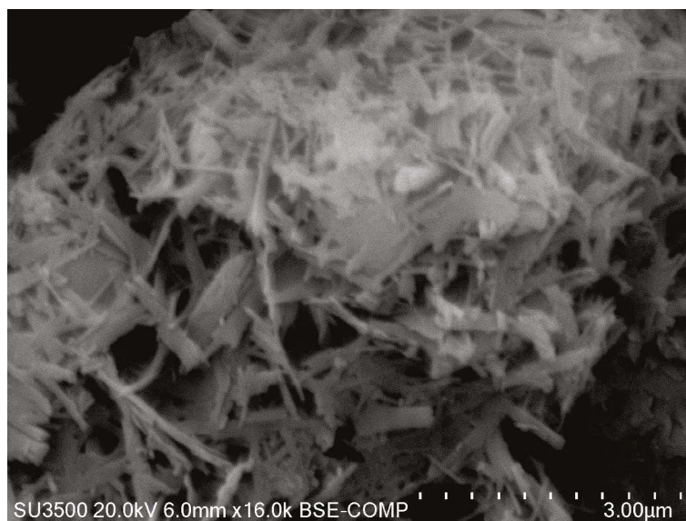
Fig. 8. SEM image of tobermorite rods and pitiglianoite bars, 16 000× magnification
