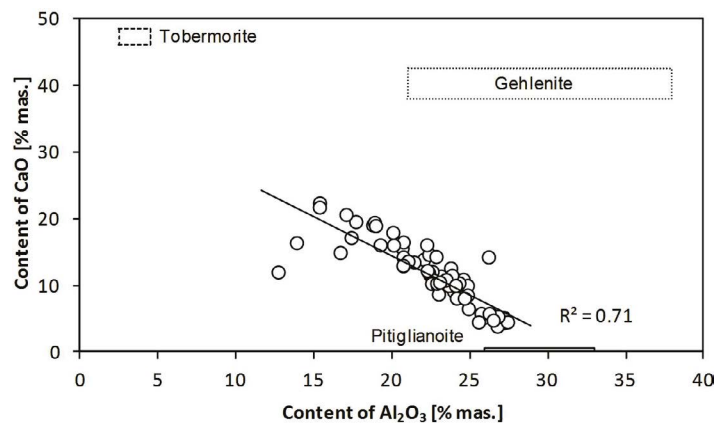
Fig. 10. Participation of Al 2 O 3 and CaO in the studied grains against the background of the theoretical differentiation of the content of these components in the tobermorite, pitiglianoite and gehlenite
