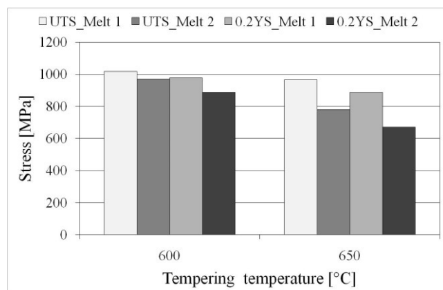
Fig. 1. Effect of tempering temperature on ultimate tensile strength (UTS) and 0.2% yield strength (0.2%YS)
