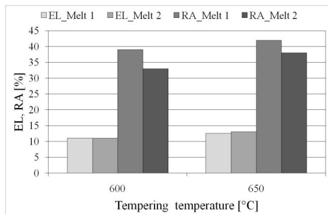
Fig. 2. Effect of tempering temperature on elongation (EL) and reduction of area (RA)
