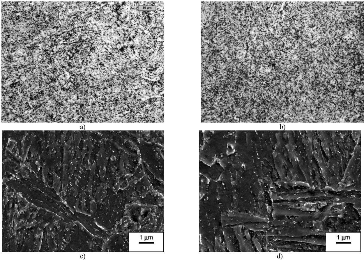
Fig. 5. Microstructure of investigated cast steels after quenching and tempering at 600 °C: a, c - melt 1 and b, d – melt 2
