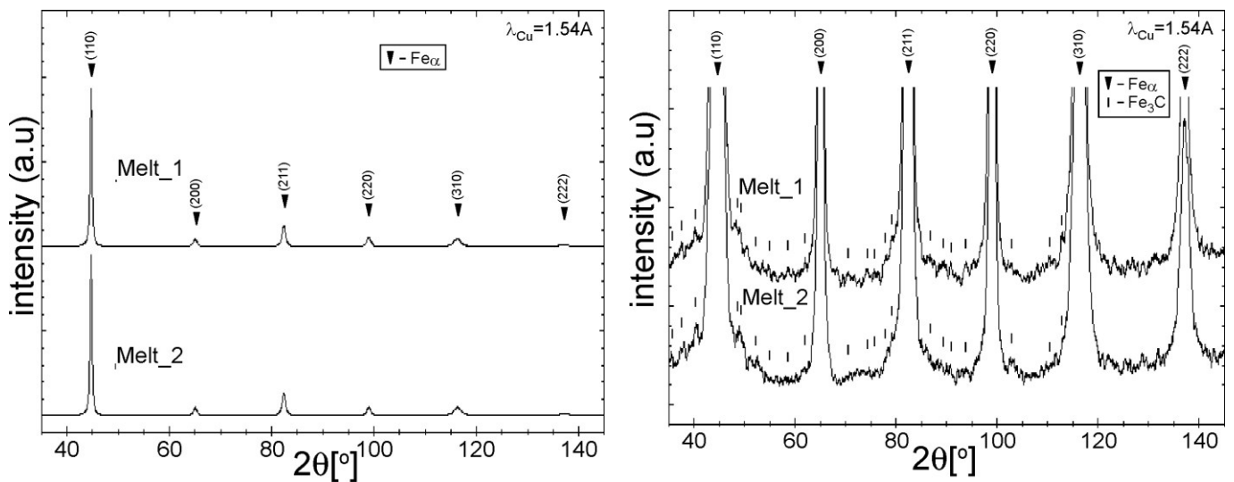
Fig. 6. The X-ray diffraction patterns of the L35HM cast steel after quenching and tempering at 600 and 650 °C
