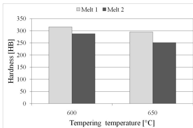
Fig. 3. The tempering temperature - hardness relationship observed in cast L35HM steel
