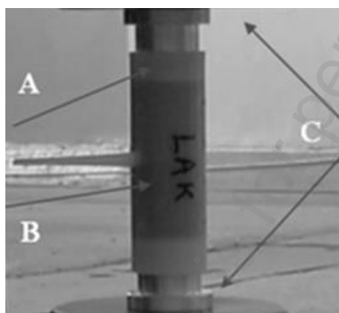
Fig. 1. Metal Oxide Surge Arrester A – insulating housing made from polyamide, B – varistor's pile, C – fittings [6]
