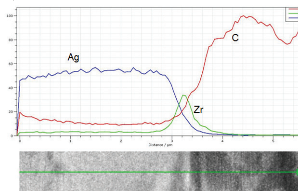
Fig. 6. SEM image of the AgZr1/ C_d interface (a) and compositional line analysis (b).
