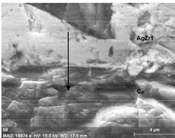
Fig. 6. SEM image of the AgZr1/ C_d interface (a) and compositional line analysis (b).
