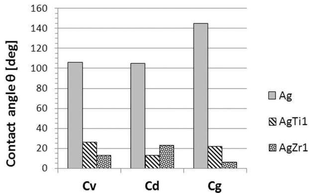
Fig. 4. Contact angles of pure Ag and its alloys AgTi1 and AgZr1 on investigated substrates ( C_v – vitreous carbon, C_d – diamond, C_g – graphite).
