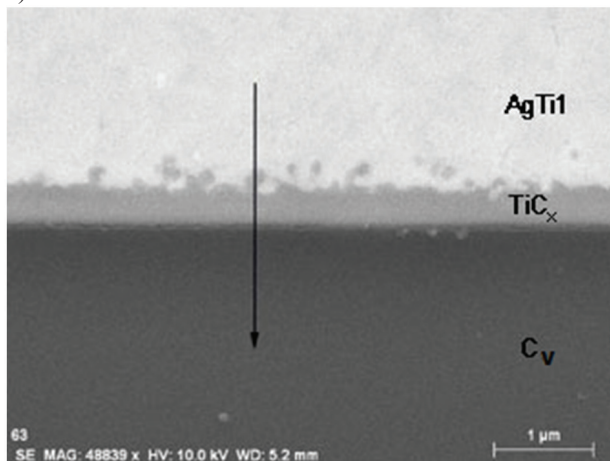
Fig. 5. SEM image of the AgTi1/ C_v interface (a) and compositional line analysis (b).
