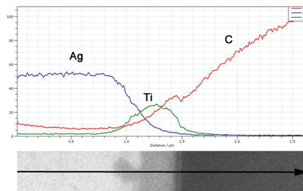
Fig. 5. SEM image of the AgTi1/ C_v interface (a) and compositional line analysis (b).
