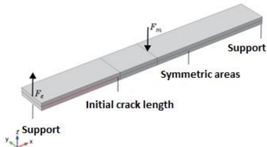
Fig. 3. Geometry of the laminate modelled [Own elaboration]
