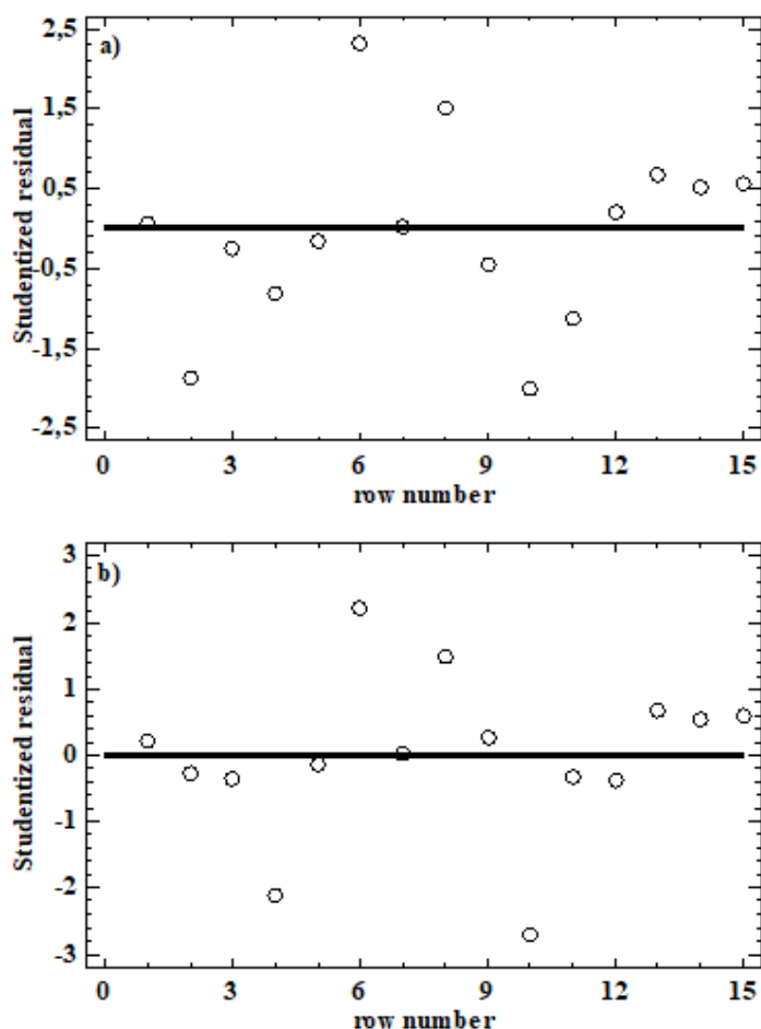
Fig. 3. Residual plots for a) FSS without constant and b) BSS without constant
