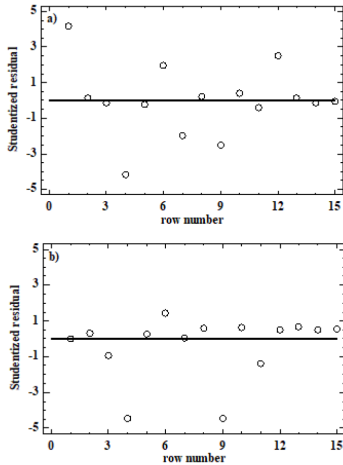
Fig. 4. Residual plots of Box-Cox transformation a) with constant and b) without constant
