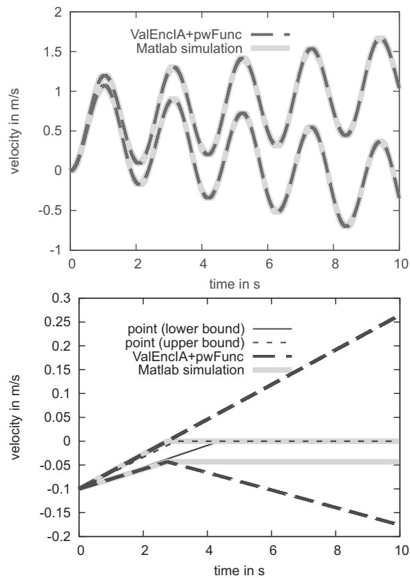
Fig. 1. Velocity of the mass for the parameter sets one (top) and two (bottom) compared with the automaton-based method.
