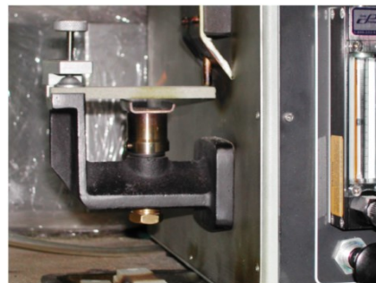
Fig. 2. Measurement module of the BCIRA test apparatus
