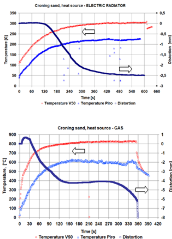
Fig. 4 Comparison of HD results and temperature changes on the bottom (by termovision camera V50) and upper (by pyrometer) surface for Croning sand (MRC). Heating by electric radiator - E (up), heating by bass burner - G (bottom)
