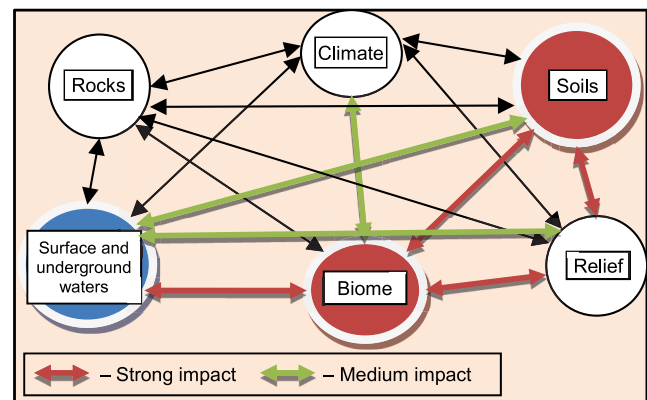
Fig. 1. Scheme of landscape functioning, systemic connections within landscapes, relationship of natural components; source: Chigarkin (1995), modified
