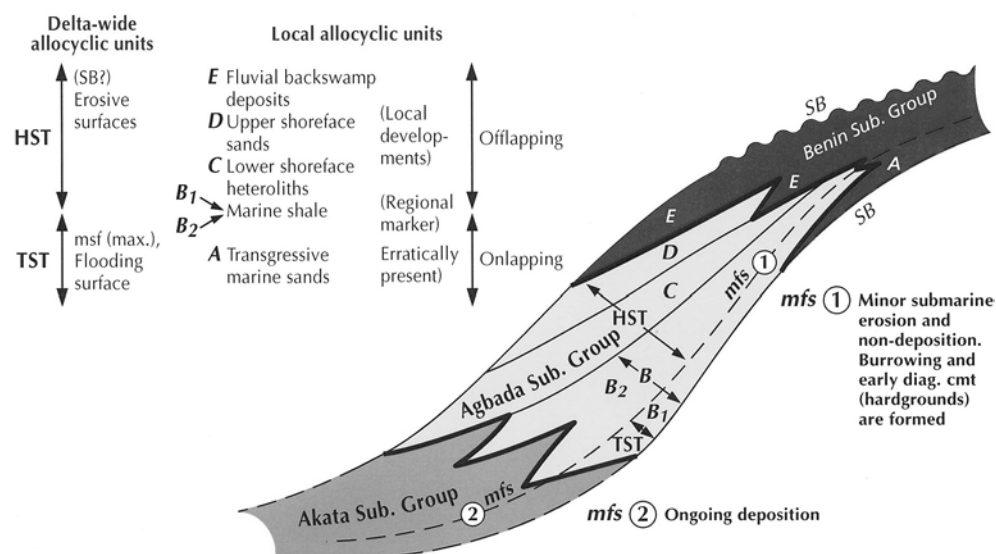
Fig. 6. Standard Vail (1987) sequence with internal allo-cyclic units in the Niger Delta.
