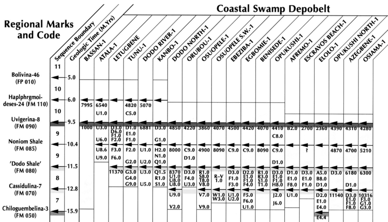
Fig. 16. Regional stratigraphic sand nomenclature for the Niger Delta (for location see Fig. 8).
