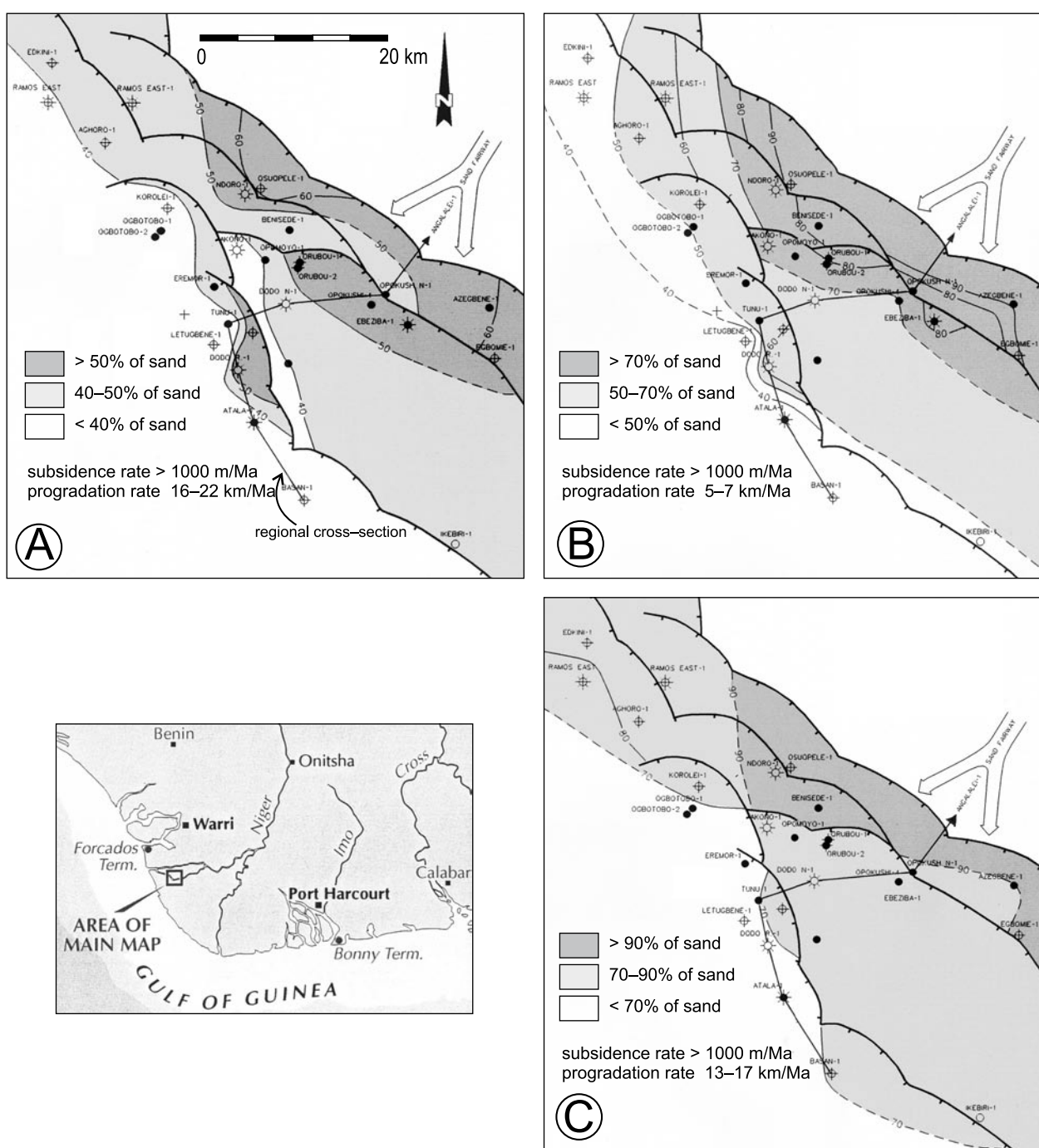
Fig. 13. Approximate sand-percentage maps in OML 35/46 (based on and modified from Edjedawe, 1981; Knox & Omatsola, 1988).
