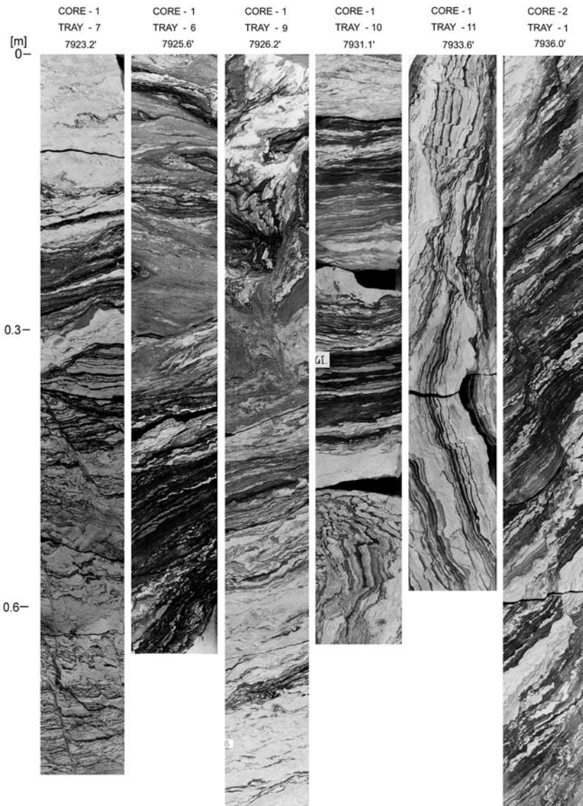
Fig. 10. The Egbema-8 core.
