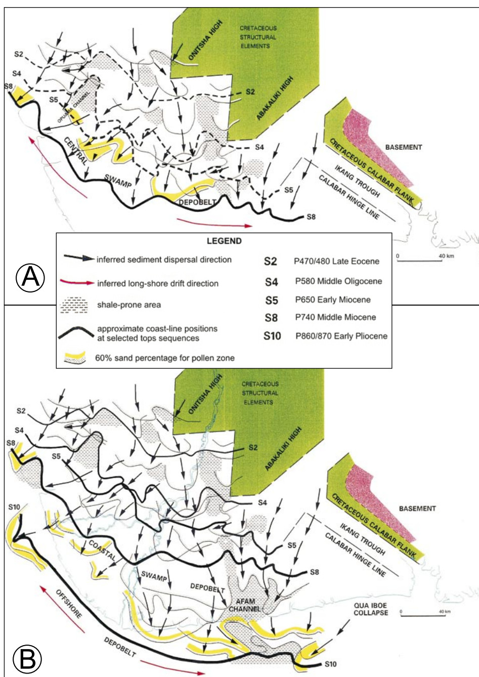
Fig. 4. Palaeo-drainage trend and advancing coastline of the Niger Delta (modified after Edjedawe, 1981; Edjedawe et al., 1984). A - Position at start of sequence 9 (Dodoshale transgression); B - Position at start of sequence 11 ( Bolivina-46 shale transgression).
