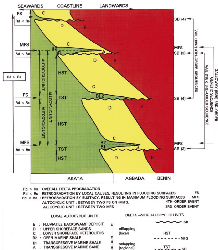
Fig. 17. Mechanisms and units of delta evolution.
