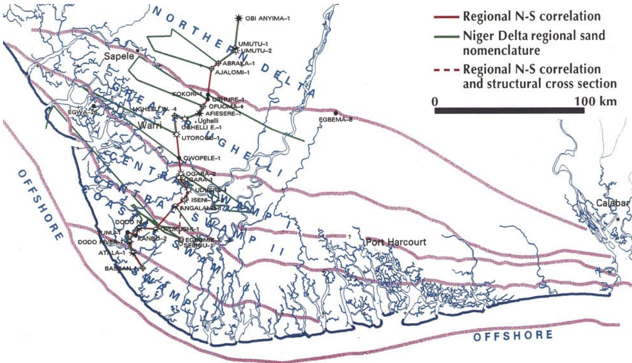
Fig. 11. Location map of depobelts, main regional trajectories and wells.
