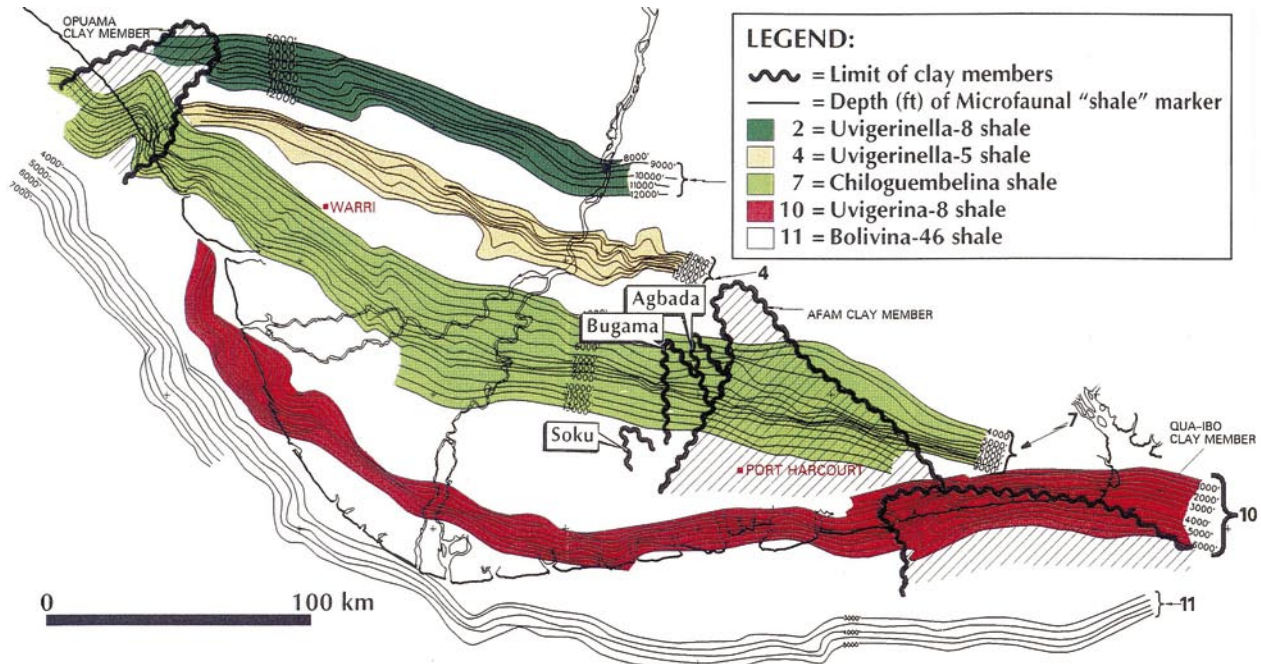
Fig. 12. Regional 3 rd -order shale markers. The ‘bands’ shown are contours of subcropping marine shales within specific depobelts (see also Fig. 8).
