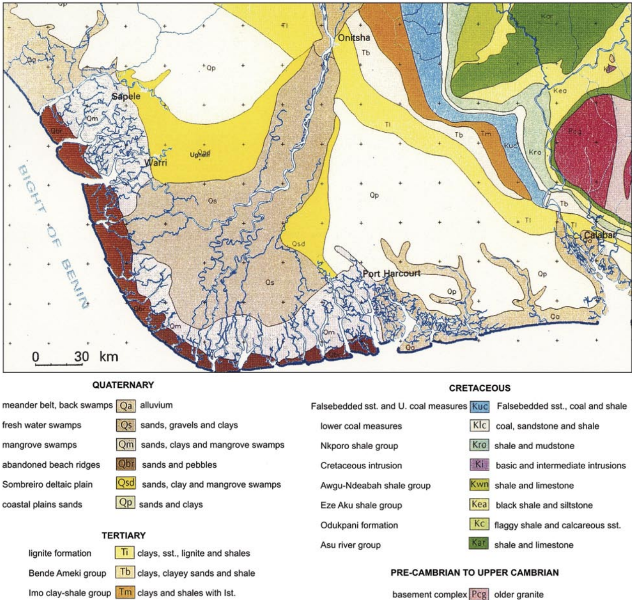
Fig. 1. Geological map of the Niger Delta and surroundings.
