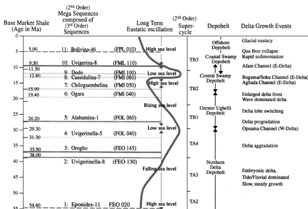
Fig. 5. Phases of delta evolution and some of their characteristics.
