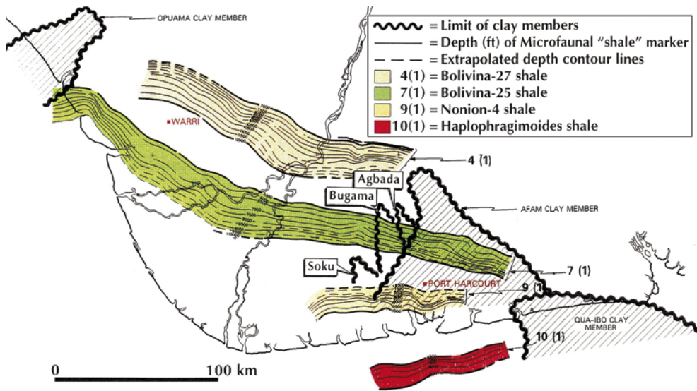
Fig. 14. Local 4 th -order shale markers. The 'bands' shown are contours of subcropping marine shales within specific depobelts (see also Fig. 8).
