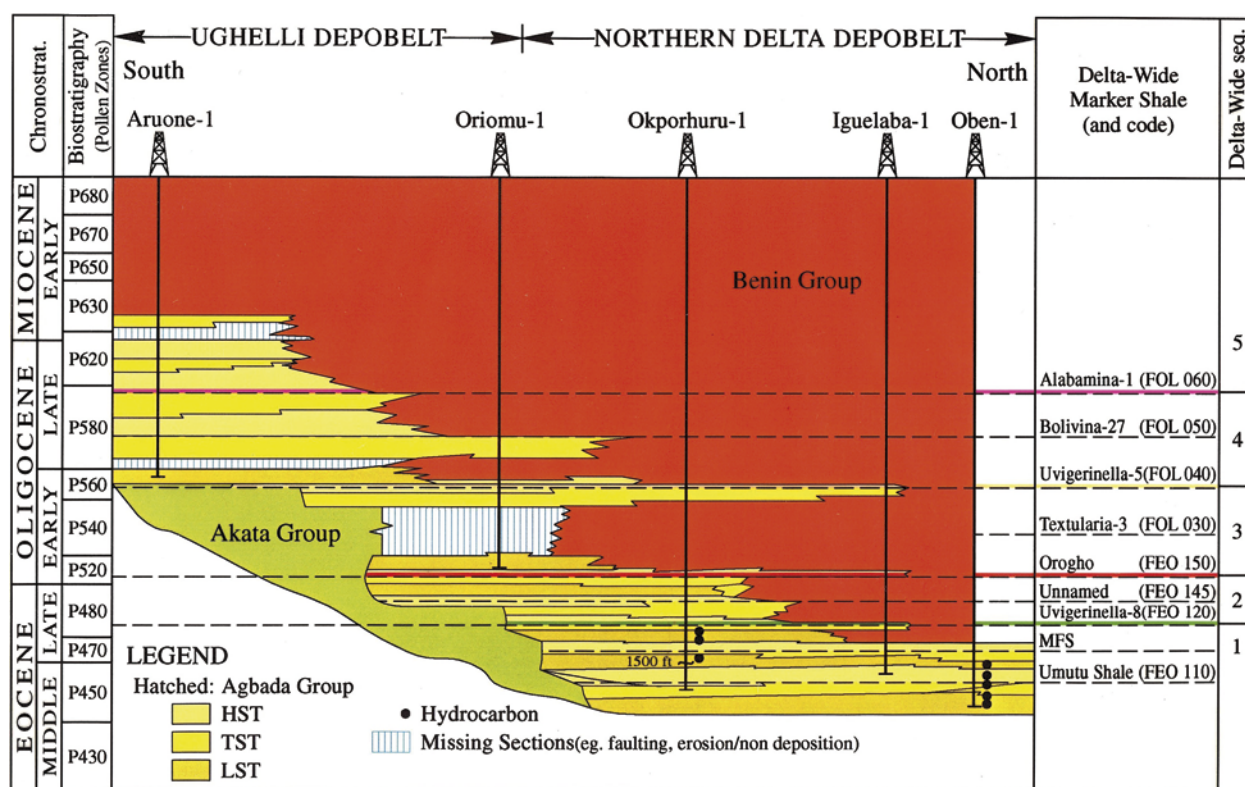
Fig. 19. Time-rock synopsis in OML-38 (Ughelli/Northern Delta depobelt).
