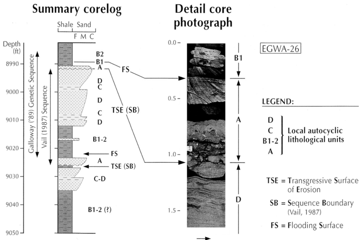
Fig. 18. 4 th -5 th -order stacked coastal barrier autocyclic lithological units.
