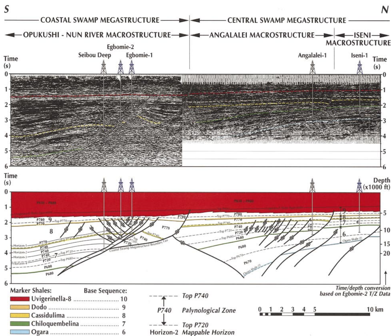
Fig. 9. Seismic section, interpretation and structural cross-section (for location see Fig. 8).
