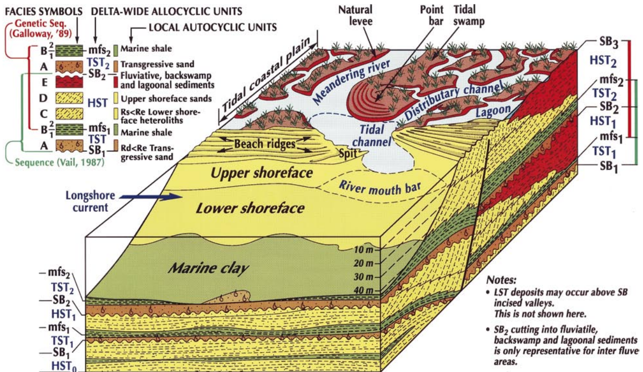
Fig. 15. Geomorphology, cyclic sedimentation and an active fault in the Tertiary Niger Delta coastal zone (modified after Weber, 1971).
