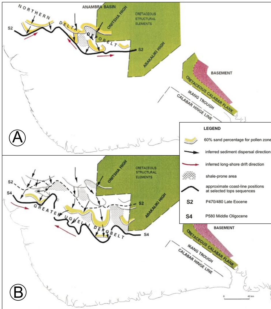
Fig. 3. Palaeo-drainage trend and advancing coastline of the Niger Delta (modified after Edjedawe, 1981; Edjedawe et al., 1984). A - Position at start of sequence 3 (Orogho-shale transgression); B - Position at start of sequence 5 ( Alabama-1 shale transgression).
