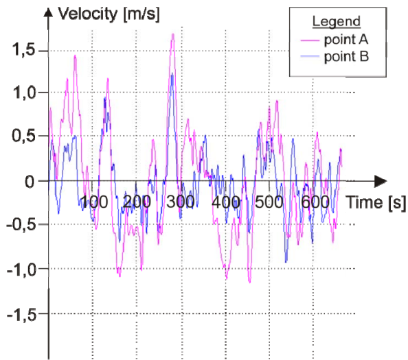
Fig.9. The graph of the wind spectrum history in the X direction according to Davenport's method.
