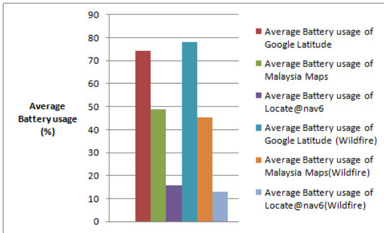
Figure 17. Application-wise average battery usage of the applications on HTC Desire and HTC Wildfire.
