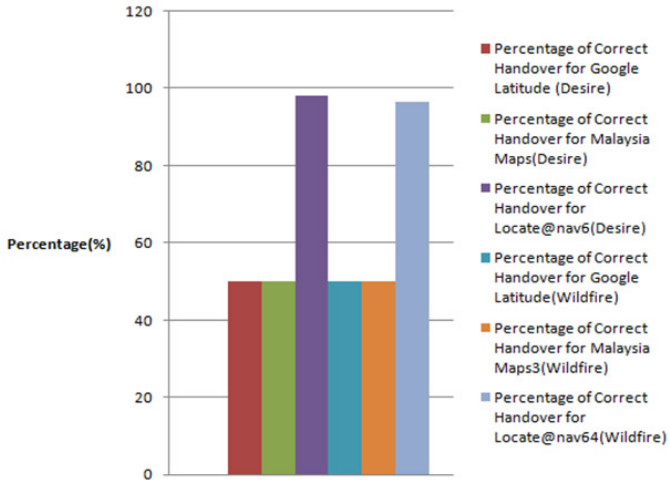
Figure 9. Percentage of correct handover for different applications on HTC Desire and HTC Wildfire.
