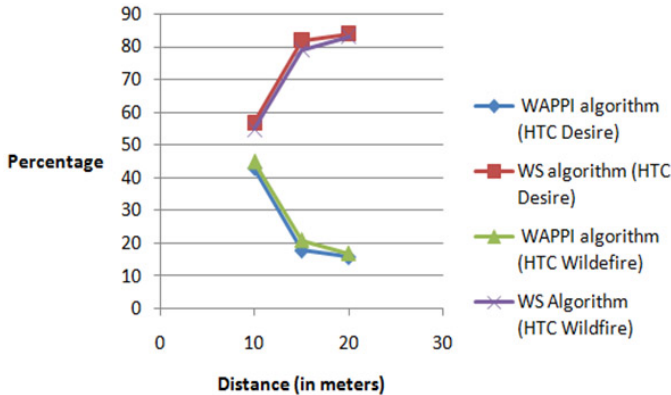
Figure 6. Distance versus percentage of usage of WAPPI and WS algorithm.
