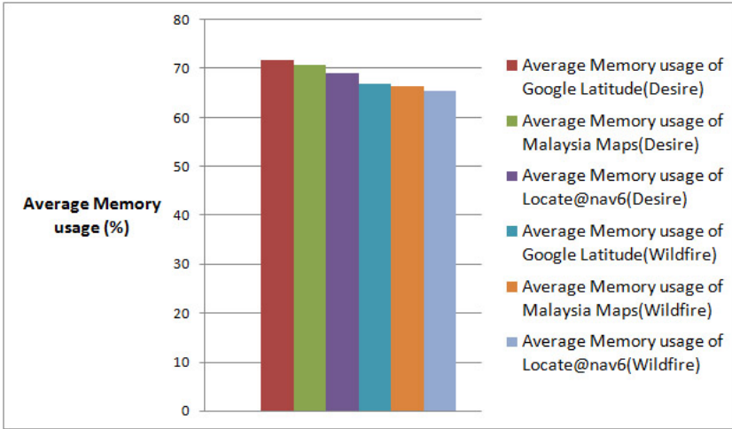
Figure 16. Percentage of average Memory usage on HTC Desire and HTC Wildfire.
