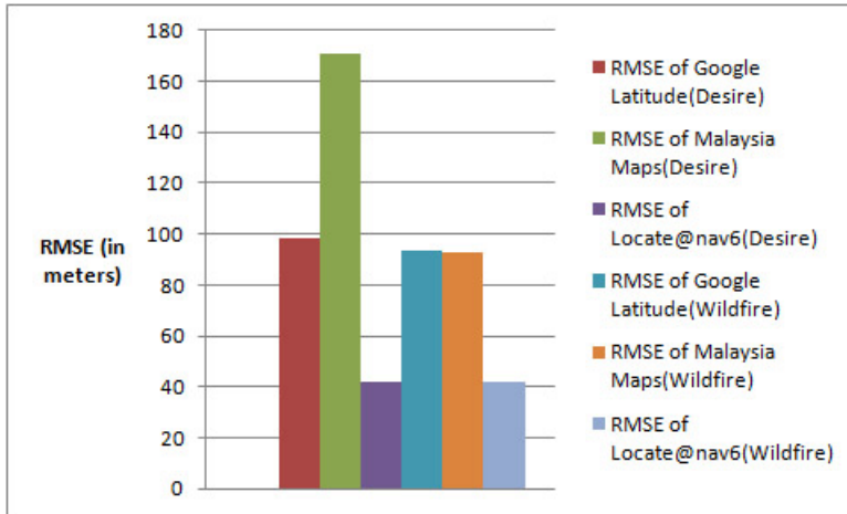
Figure 14. RMSE of positioning for the applications on HTC Desire and HTC Wildfire.
