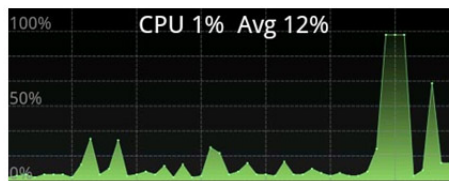
Figure 20. Runtime CPU usage for Locate@nav6 on HTC Desire.
