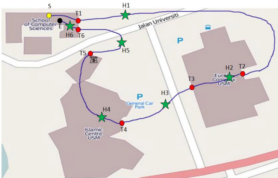
Figure 8. Handovers performed by Locate@nav6 on HTC Desire during experiment.
