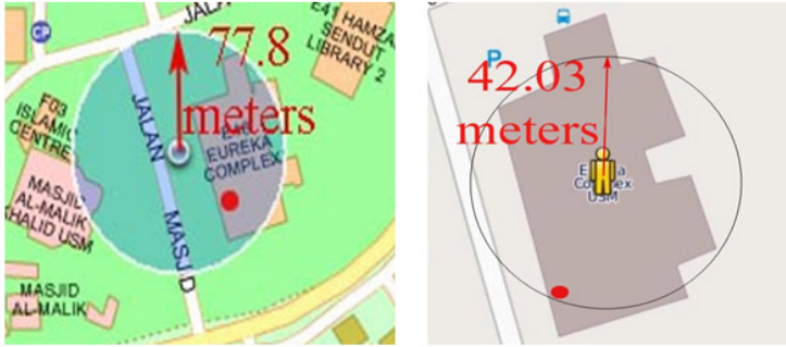
Figure 13. Samples showing actual and estimated position of Malaysia maps (left) and Locate@nav6 (right) during handover on HTC Wildfire.
