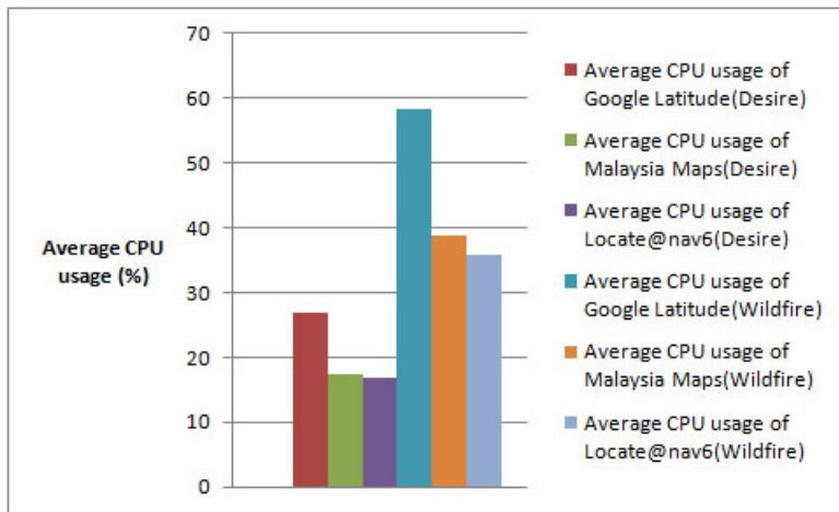
Figure 15. Percentage of average CPU usage on HTC Desire and HTC Wildfire.
