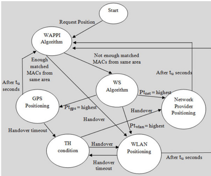
Figure 3. State diagram of proposed design.
