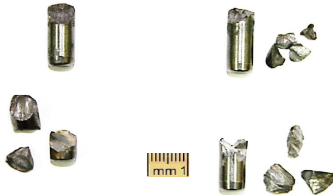
Fig. 16. Bullet core after normal perforation of 8 mm thickness plates
