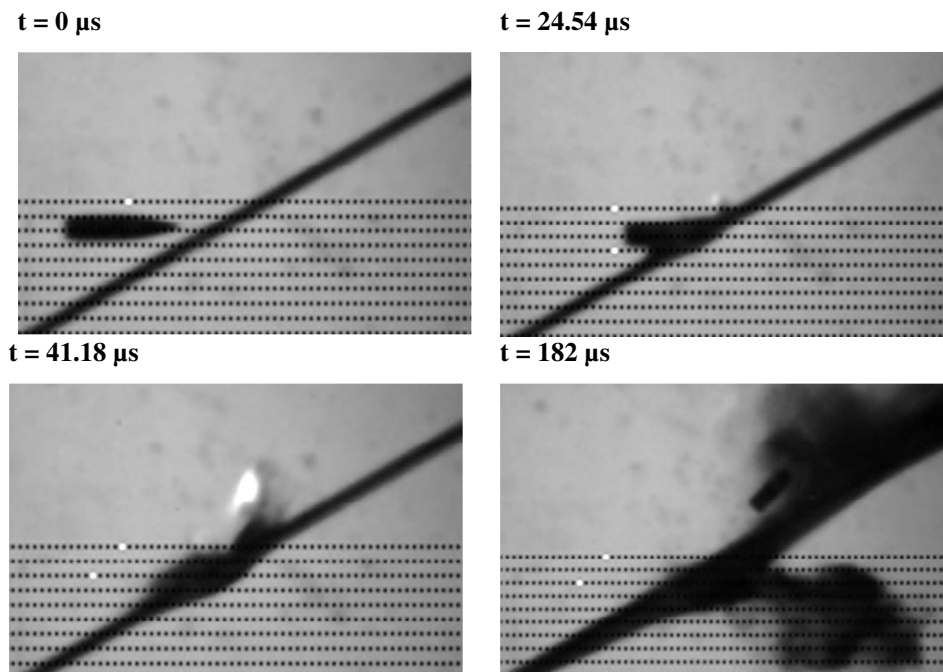
Fig. 22. High speed camera images of 60° oblique perforation tests of 3 mm thickness 30PM steel plates
