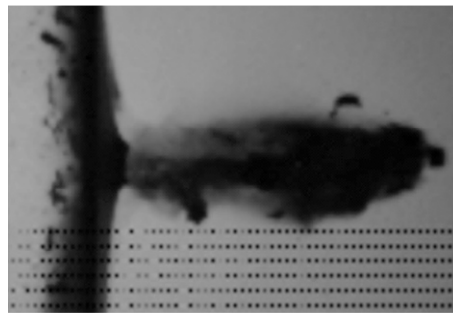
Fig. 8. High speed camera images of perforation tests of 3 mm thickness 30PM steel plates
