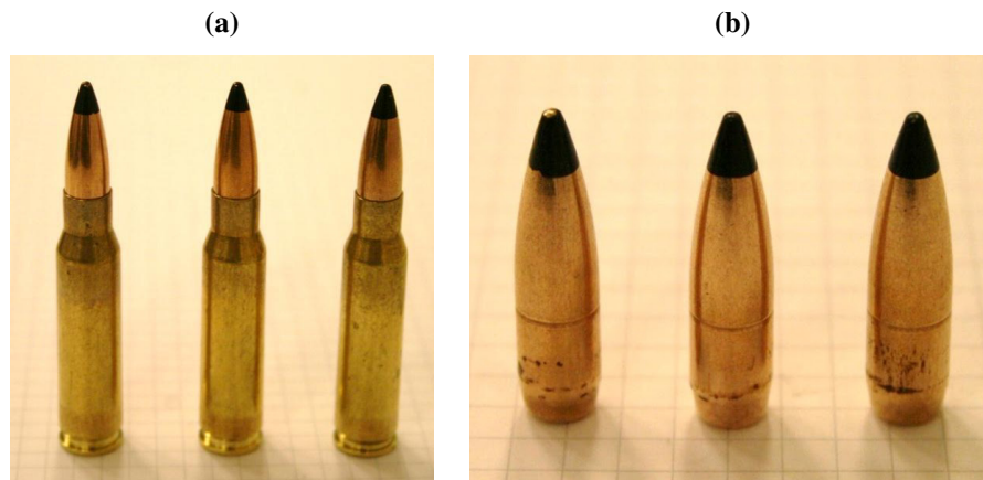
Fig. 1. Ammunition (a) and the antitank (AP) projectiles (b)
