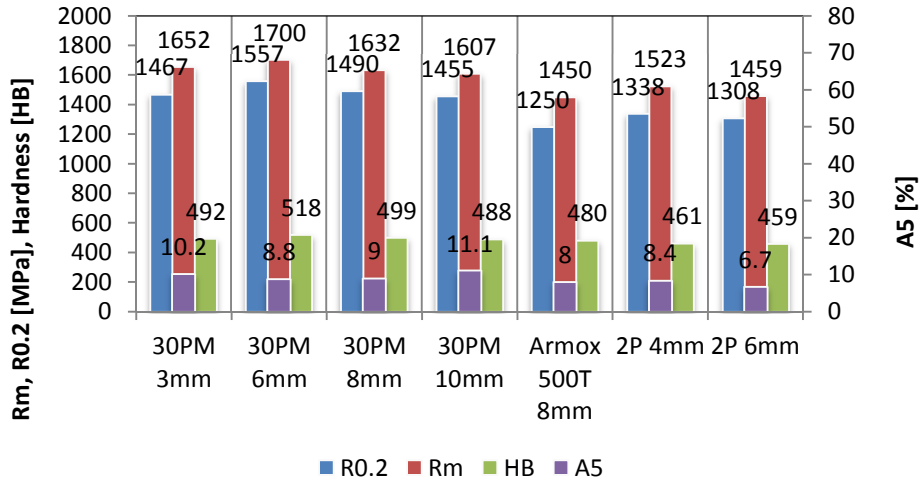
Fig. 6. Comparison of mechanical properties of 30PM armor plates with Armox 500T and 2P steel
