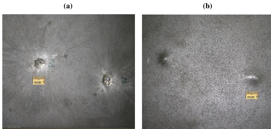
Fig. 15. 30PM steel plates of 8 mm thickness after normal perforation tests (a) impact surface (b) rear surface
