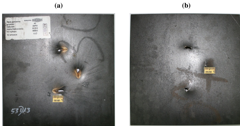
Fig. 23. 30PM steel plates of 3 mm thickness after 60° oblique perforation tests (a) impact surface (b) rear surface
