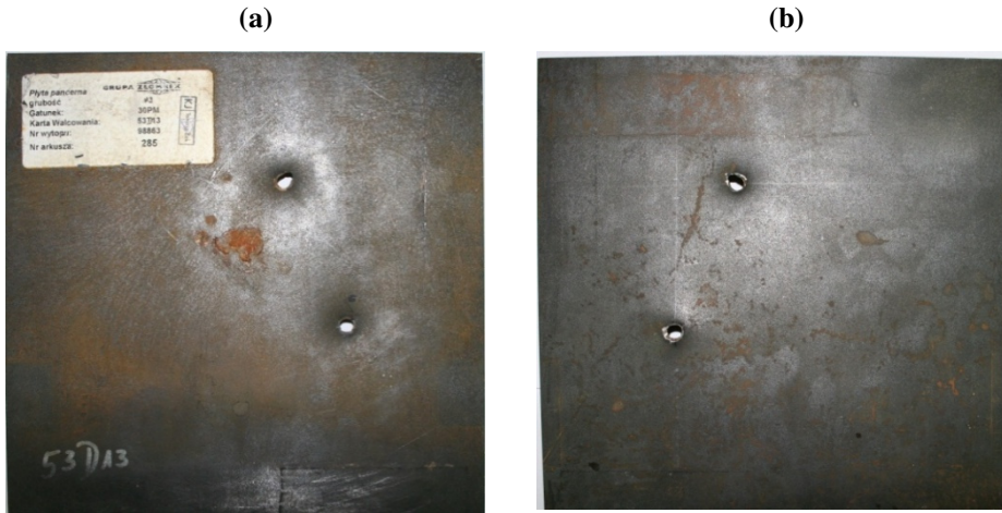
Fig. 7. 30PM steel plates of 3 mm thickness after normal perforation tests (a) impact surface (b) rear surface
