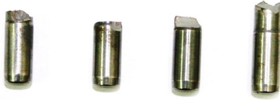
Fig. 9. N12E Bullet core after normal perforation tests of 3 mm thickness plates
