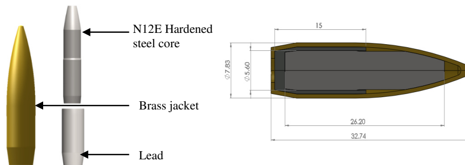
Fig. 2. Schematic drawing geometry of 7.62 mm AP bullet
