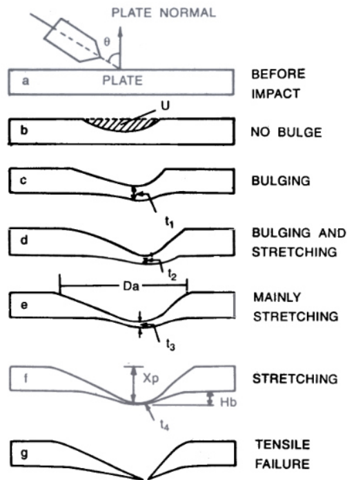
Fig. 20. Plate behaviour with some parameters studied in oblique situation
