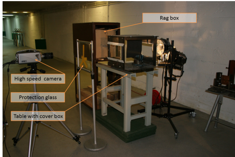
Fig. 5. Recording system used during shot tests
