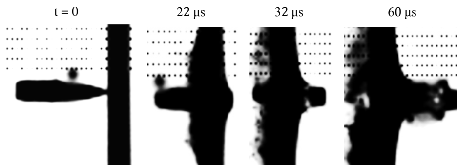
Fig. 13. High speed camera images of perforation tests of 6 mm thickness 30PM steel plates
