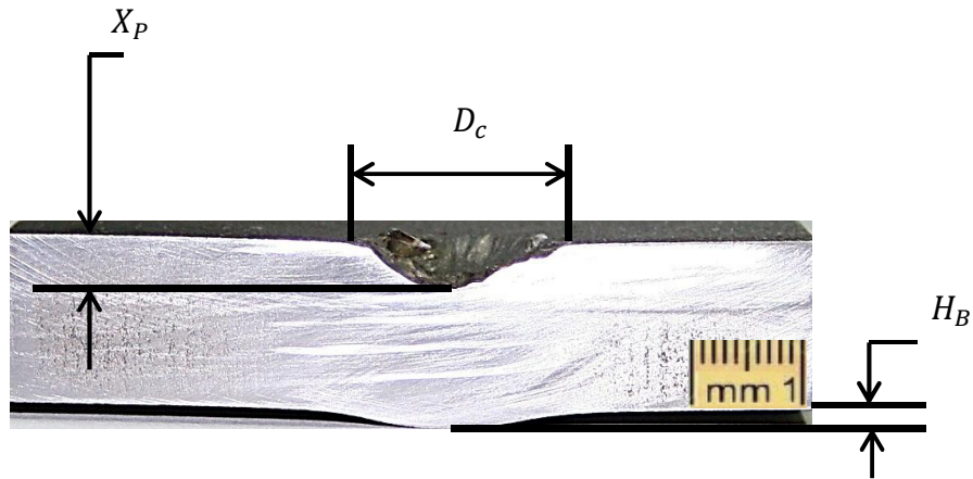
Fig. 17. Cross section of 8 mm plates subjected to normal impact by 7.62 AP projectile with some parameters used in the study
