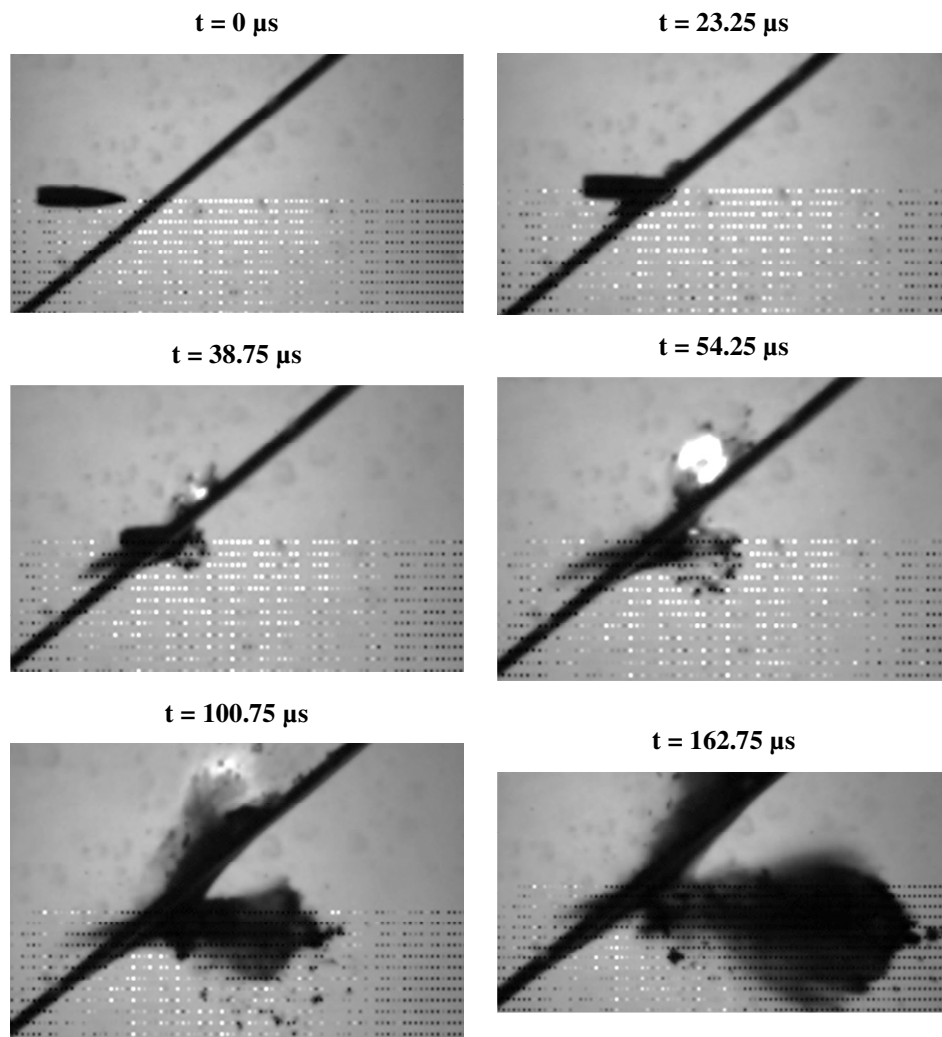
Fig. 19. High speed camera images of 50° oblique perforation tests of 3 mm thickness 30PM steel plates
