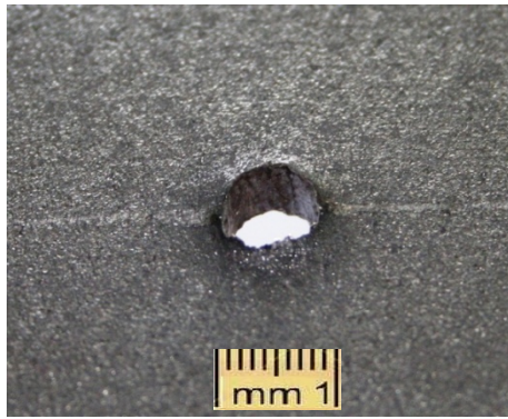
Fig. 11. Generated hole of 6.4 mm 30PM steel plate subjected to blunt-ogival hardened steel core
