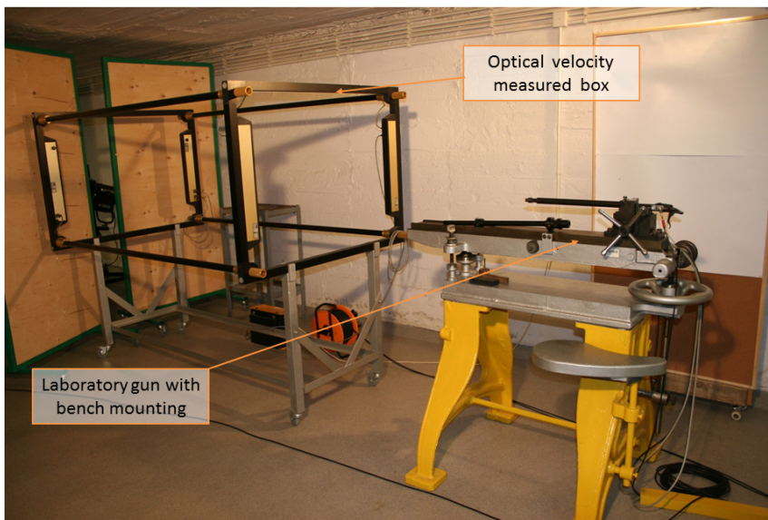
Fig. 4. Laboratory gun and optical velocity measurement system
