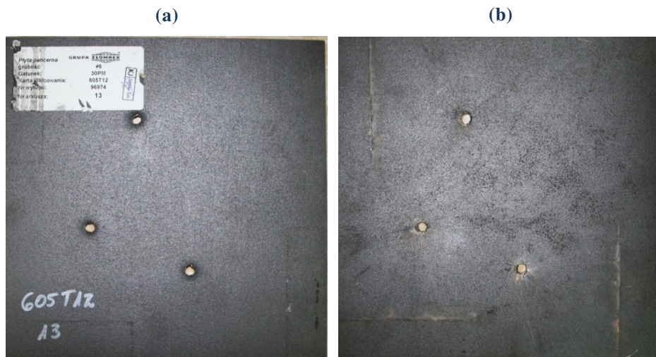
Fig. 10. 30PM steel plates of 6 mm thickness after normal perforation tests (a) impact surface (b) rear surface
