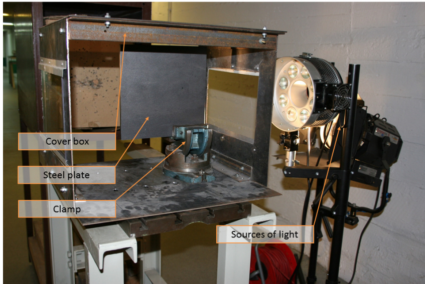
Fig. 3. Target plate mounting system
