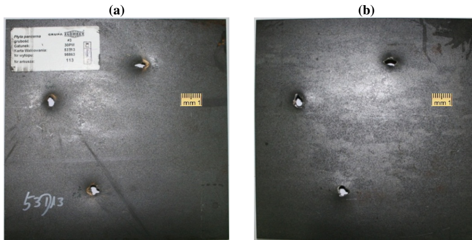
Fig. 18. 30PM steel plates of 3 mm thickness after 50° oblique perforation tests (a) impact surface (b) rear surface
