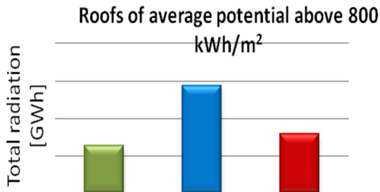
Fig. 7. Total annual solar radiation [GWh] for roofs of average potential above 800 kWh/m 2 in three analysed areas
