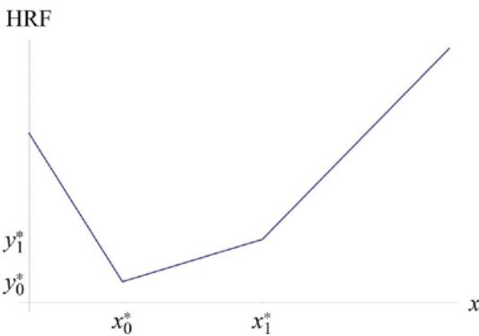
Fig. 1. Exemplary plot of the introduced HRF
