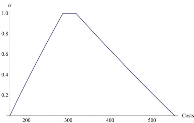
Fig. 9. Fuzzy approximation of the present value of the maintenance costs PV(cost)
