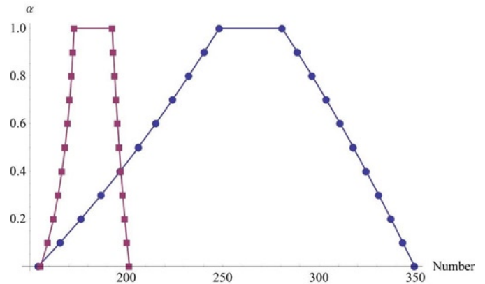
Fig. 10. Fuzzy approximation of the average number of repairs \bar{x}_R for P^* = 5 (years, circles) and P^* = 20 (years, rectangles)
