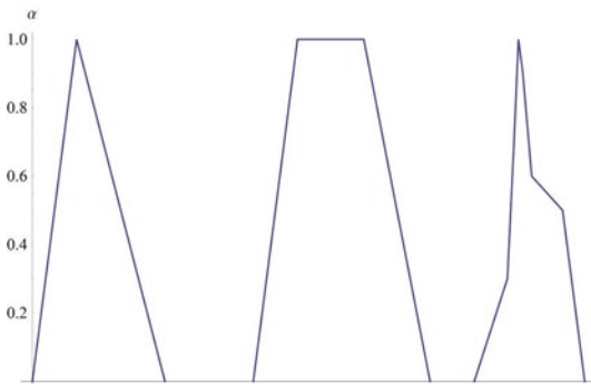
Fig. 4. Examples of fuzzy numbers (the left-hand side to the right-hand side: a triangular fuzzy number, a trapezoidal fuzzy number, a left-right fuzzy number)
