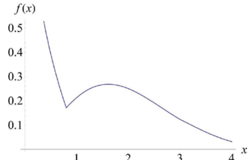
Fig. 2. Exemplary plot of the density for the introduced HRF
