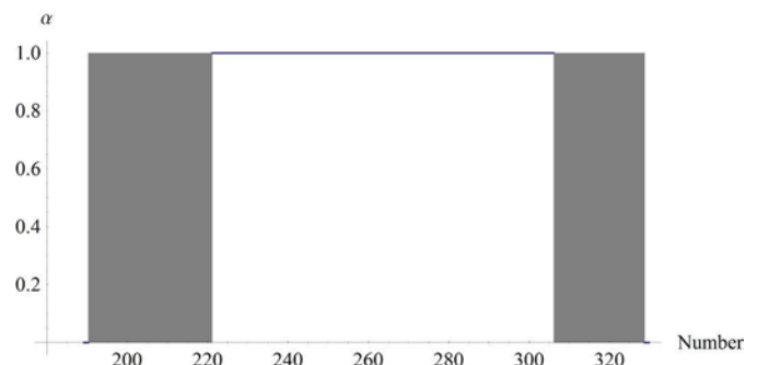
Fig. 15. Shadowed set approximation of the present value of the maintenance costs PV(cost) .
