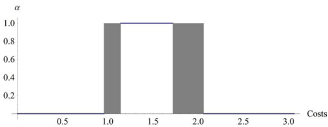
Fig. 12. Shadowed set approximation of the mean of the repairs costs
