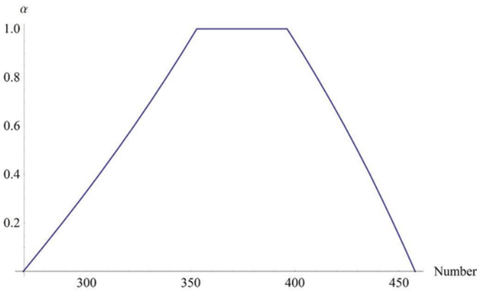
Fig. 8. Fuzzy approximation of the average number of repairs \bar{x}_R
