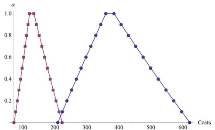
Fig. 11. Fuzzy approximation of the present value of the maintenance costs PV(cost) for P^* = 5 (years, circles) and P^* = 20 (years, rectangles)
