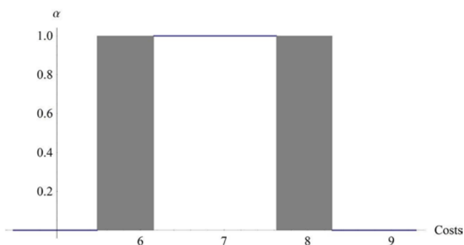
Fig. 13. Shadowed set approximation of the mean of the replacements costs
