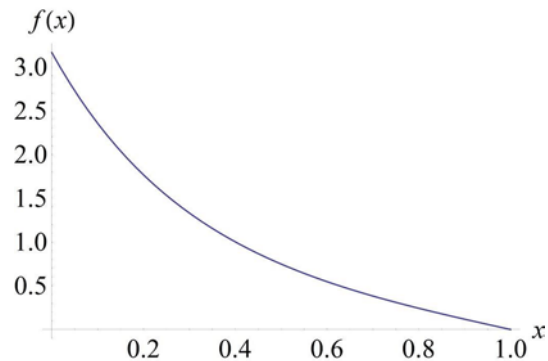
Fig. 3. Exemplary plot of the density for the repairing and the replacement times
