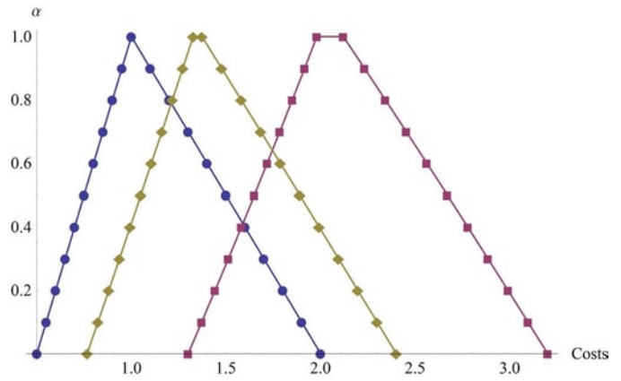
Fig. 6. Fuzzy approximations of the minimum (circles), the mean (diamonds), and the maximum (rectangles) of the repairs costs
