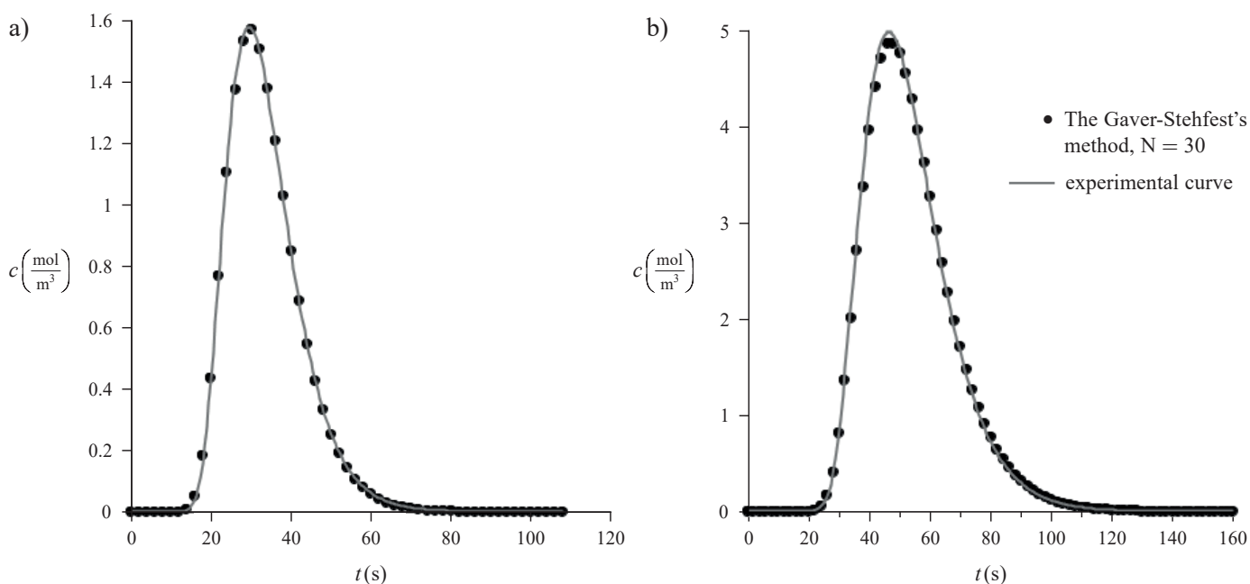
Fig. 2. Numerical and experimental profiles of gas concentration: a) P = 1.20 \cdot 10^5 Pa, T = 333 K, V_{imp} = 2.50 \cdot 10^{-7} m 3 , F_v = 3.33 \cdot 10^{-7} m 3 /s, t_p = 0.75 s; b) P = 2.00 \cdot 10^5 Pa, T = 353 K, V_{imp} = 5.00 \cdot 10^{-7} m 3 , F_v = 3.33 \cdot 10^{-7} m 3 /s, t_p = 1.50 s
