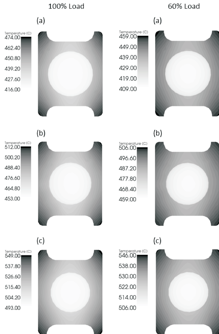
Figure 3. Temperature distribution at the outlet cross section of the first (a), second (b), and third (c) pass of a superheater for 100% and 60% loads.
