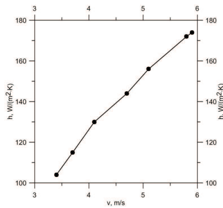
Figure 7. The heat transfer coefficient as a function of the flue gas velocity.
