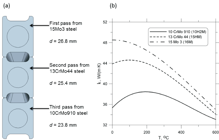
Figure 2. Three passes made from different steels and with different inner diameters (a) and thermal conductivity coefficients as a function of temperature (b).
