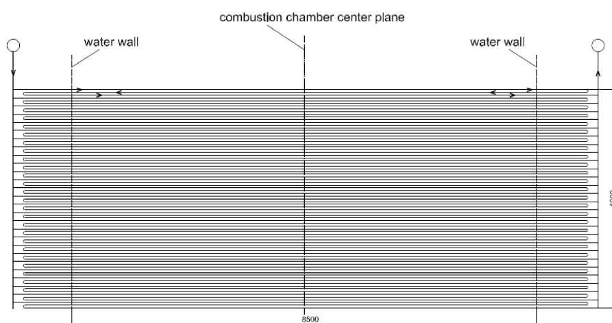
Figure 1. The platen which includes 81 serial tubes forms the 27 three-pass tube sets.
