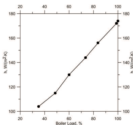
Figure 5. The heat transfer coefficient as a function of the boiler load.
