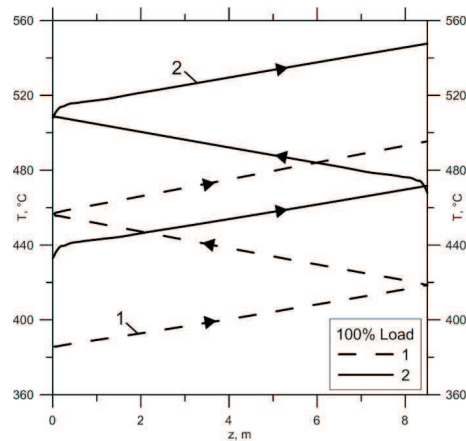
Figure 4. Changes in mass average steam temperature and tube wall temperature at the tube corner along the steam flow path: 1 – steam; 2 – tube wall temperature at the corner.
