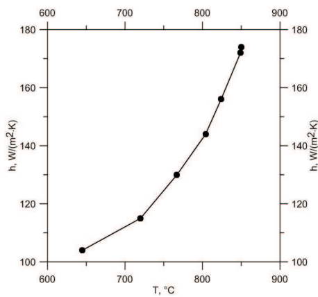
Figure 6. The heat transfer coefficient as a function of the flue gas temperature.
