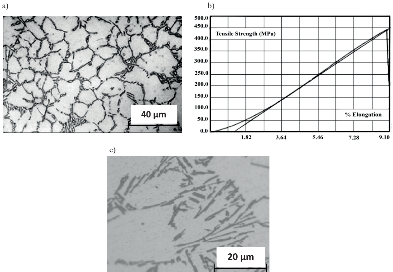
Fig. 4. a) Microstructure of as-cast Al-6%Si alloy before refinement. Coarse Si phase homogeneously distributed without aggregation. The size of the Si phase and the grains are about 10 \mu m and 35-40 \mu m. b) Tensile curve at strain rate of 10 -1 s -1 in room temperature. The maximum strength is about 430MPa and fracture occurred at the elastic limit with 8.9% elongation. c) The same microstructure with more magnification. The needle-plate like eutectic silicon is distributed arbitrarily in the Al matrix.
