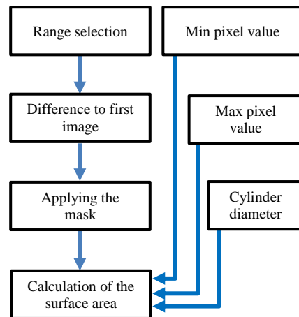
Fig. 4. Optical analysis algorithm using DaVis 7.2
