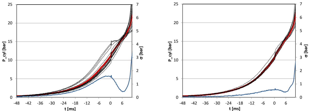
Fig. 3. Sequences of indicated pressure P_{cyl} (black), mean value (red) and standard deviation (blue) for the compression curve using conventional ignition. On the left before the selection, on the right after the exclusion of incorrect RCM work cycles; the characteristic peak on the pressure curve was caused by interferences from the ignition system ( t = 0 ms)
