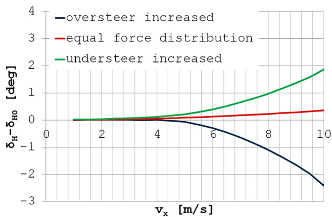
Fig. 8. Steering characteristic of nontilting vehicle with driving forces differentiation
