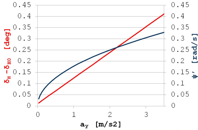
Fig. 6. Steering characteristic of the nontilting vehicle with equal force distribution
