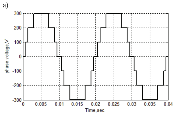
Fig. 6. a) Simulation results of a 7-level multilevel inverter for output phase voltage; b) Simulation results of a 7-level multilevel inverter, FFT analysis for phase voltage
