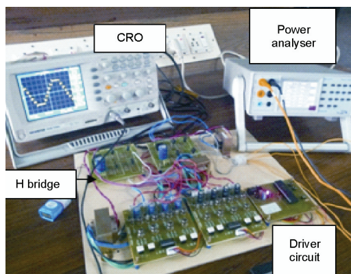
Fig. 8. The hardware prototype
