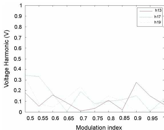
Fig. 4. Modulation index, M and higher order harmonics h13, h17 and h19 for seven level hybrid cascaded multilevel inverter in WTHD approach
