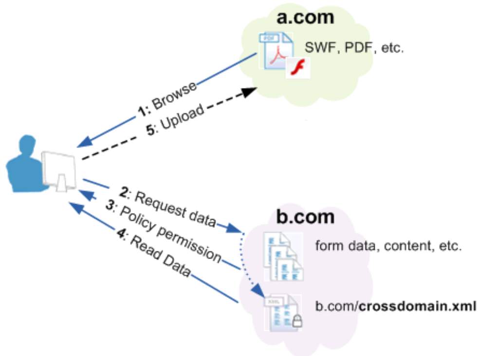
Figure 4 Explanation of Cross-Domain Policy
