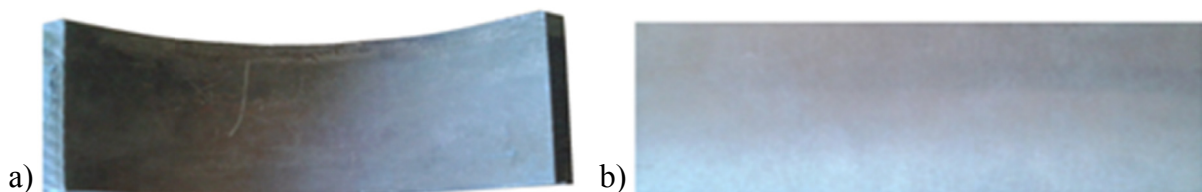
Fig. 4. View of sheets after rolling process a) symmetrical, b) asymmetrical a_v = 0.75
