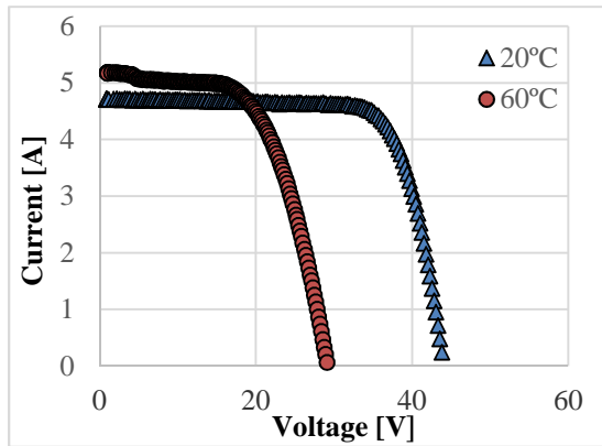
Fig. 11a. The I-V characteristics of PV module under different cell temperatures (20 and 60°C) for light concentration of 1000 W/m 2 .
