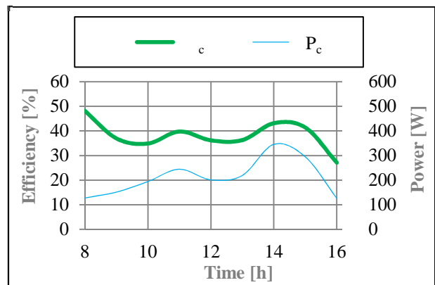
Fig. 5b. Instantaneous power and efficiency values of solar thermal collector.
