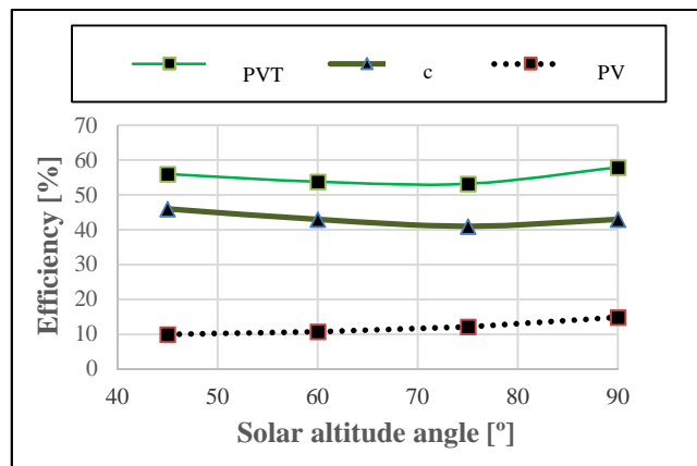
Fig. 10b. Efficiency measured under laboratory conditions. Source: Author's
