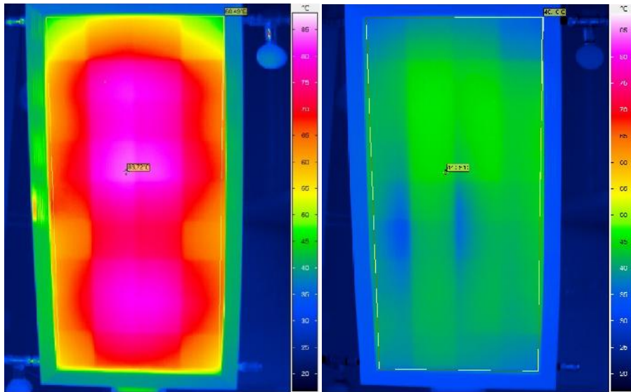
Fig. 11c. Solar hybrid system working without liquid flow (left) solar hybrid system after 15 minutes of liquid flow (right).
