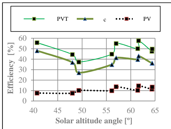
Fig. 10a. Efficiency measured under field conditions. Source: Author's
