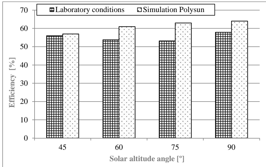
Fig. 10c. PVT collector efficiency under laboratory conditions and corresponding Polysun simulation results Source: Author's
