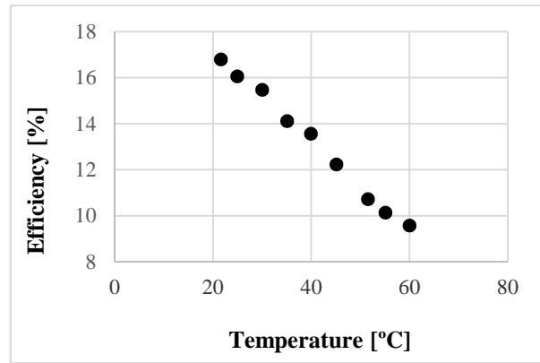
Fig. 11b. The effect of temperature increase on PV module efficiency for light intensity 1000 W/m 2 .
