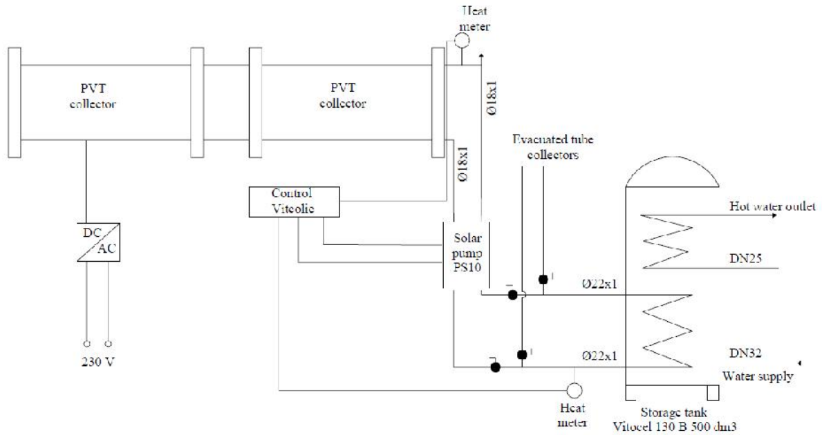
Fig. 2. Schematic diagram of installation PVT collectors.
