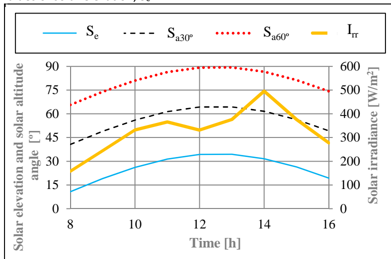
Fig. 3. The solar irradiance measured during field experiment, solar elevation and calculated solar altitude angle.
