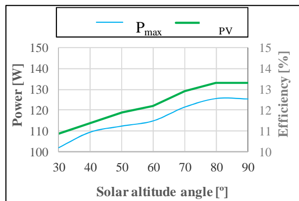
Fig. 8b The power ( P_{\max} ) and efficiency ( \eta_{PV} ) as function of altitude angle for \Delta T = 30^\circ\text{C} .
