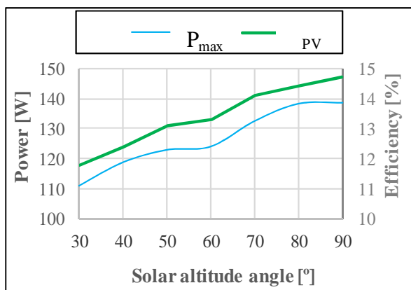
Fig. 8a. The power ( P_{\max} ) and efficiency ( \eta_{PV} ) as function of altitude angle for \Delta T = 5^\circ\text{C} .
