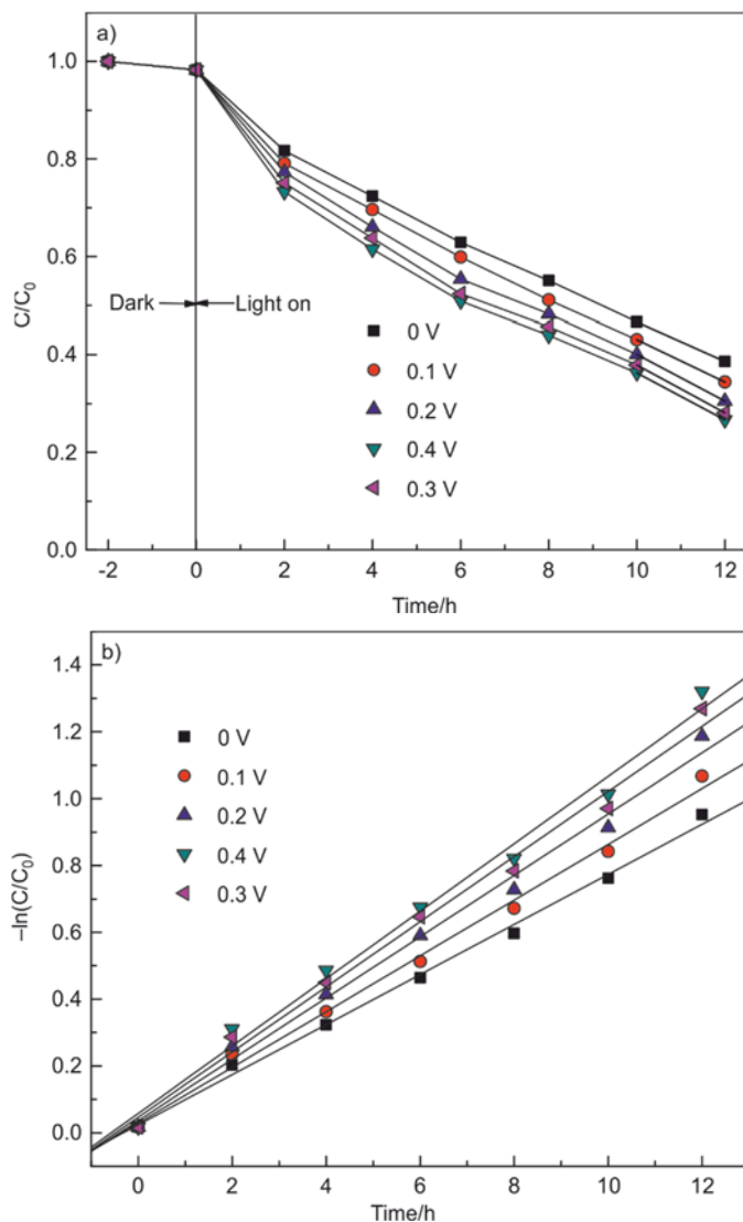
Fig. 4. Effect of external potential on the PEC degradation of diclofenac (a) and evolution curves (b) by N, S-TiO 2 NCs/TiO 2 NTAs photoelectrode; diclofenac initial concentration 5 mg·dm -3 , Na 2 SO 4 concentration 0.10 mol·dm -3 , pH 5
