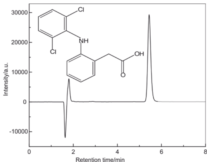
Fig. 1. High performance liquid chromatogram spectrum of diclofenac solution (5mg·dm -3 )
