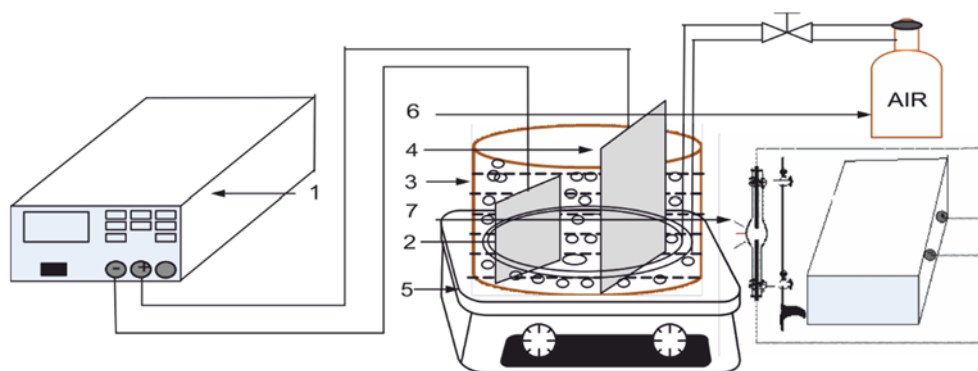
Fig. 2. Schematic diagram for PEC reaction: 1 – DC power supply, 2 – Pt cathode, 3 – quartz reactor, 4 – \text{TiO}_2 NTas photoanode, 5 – magnetic stirrer, 6 – air aerator, 7 – xenon lamp
