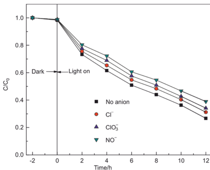
Fig. 8. Effect of various anions ( 0.05 \text{ mol}\cdot\text{dm}^{-3} ) of on the PEC degradation of diclofenac by N, S- \text{TiO}_2 NCs/ \text{TiO}_2 NTAs photoelectrode; initial diclofenac concentration 5 \text{ mg}\cdot\text{dm}^{-3} , \text{Na}_2\text{SO}_4 concentration 0.10 \text{ mol}\cdot\text{dm}^{-3} , pH 5.0, external potential 0.4 V (vs. SCE)
