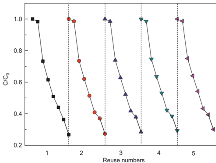
Fig. 9. Cycling runs in the PEC degradation of diclofenac solution in the presence of N, S-TiO 2 NCs/TiO 2 NTAs photoelectrode under 35 W Xenon light irradiation; initial diclofenac concentration 5 mg·dm -3 , Na 2 SO 4 concentration 0.10 mol·dm -3 , pH 5.0, external potential 0.4 V (vs. SCE)
