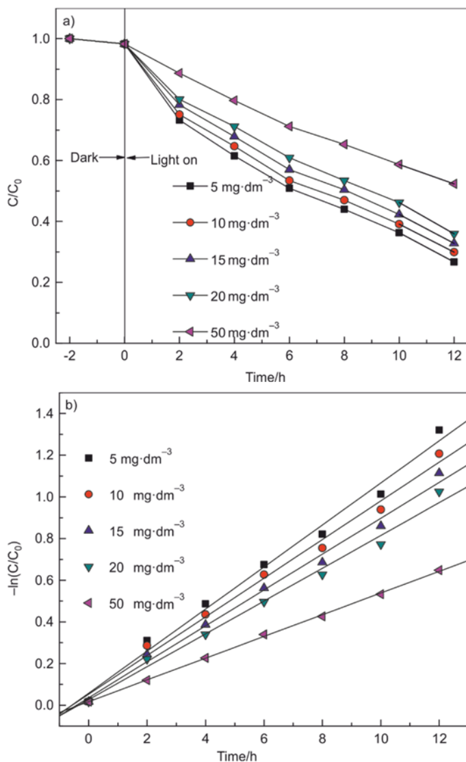
Fig. 6. Effect of initial concentration of diclofenac on the PEC performance (a) and evolution curves (b) by N, S-TiO 2 NCs/TiO 2 NTAs photoelectrode; Na 2 SO 4 concentration 0.10 mol·dm -3 , pH 5.0, external potential 0.4 V (vs. SCE)
