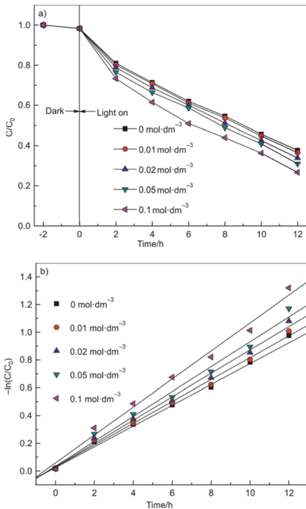
Fig. 5. Effect of concentration of sodium sulfate on the PEC degradation of diclofenac (a) and evolution curves (b) by N, S-TiO 2 NCs/TiO 2 NTAs photoelectrode; initial diclofenac concentration 5 mg·dm -3 , pH 5, external potential +0.4 V (vs. SCE)
