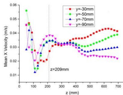
Fig. 12. Tangential velocity distribution along the axial direction on the iso-surface of y = -90 mm, -70 mm, -50 mm, -30 mm ( x = 0 mm, z = 50 – 700 mm)
