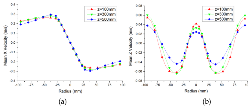
Fig. 8. Velocity distribution within the column flotation unit at different heights. (a) Mean tangential velocity and (b) mean axial velocity.
