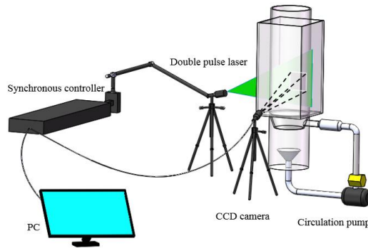
Fig. 2. Experimental setup
