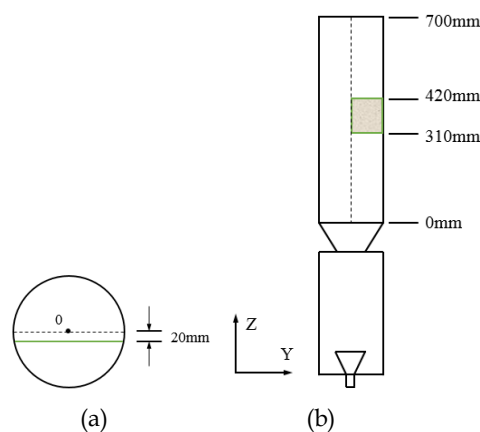
Fig. 3. Schematic of PIV measurement area. (a) Measured plane and (b) measured region
