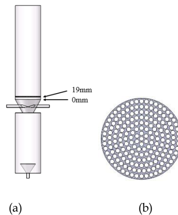
Fig. 9. Schematic of sieve-plate packing. (a) Configurations of one layer of sieve-plate packing and (b) geometry of the sieve plate.
