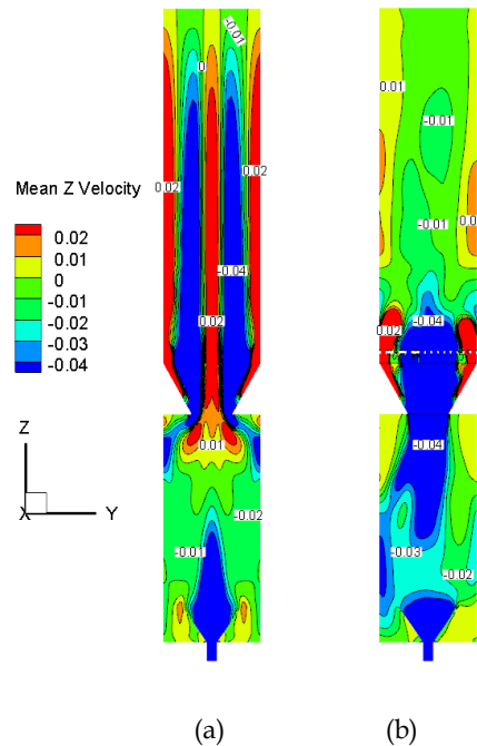
Fig. 11. Contour of mean z velocity on plane of x = 0 mm. (a) Open column and (b) one layer of sieve-plate packing
