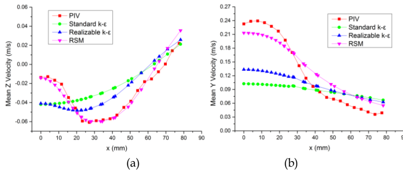
Fig. 6. Velocity distribution on line z = 365 mm (y = 20 mm); (a) mean axial velocity and (b) mean radial velocity
