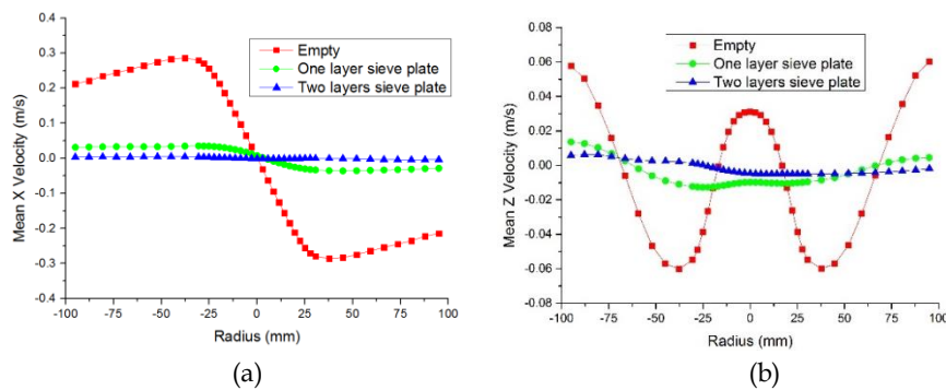
Fig. 14. Velocity distribution at z = 365 mm ( x = 0 ). (a) Mean x velocity and (b) mean z velocity
