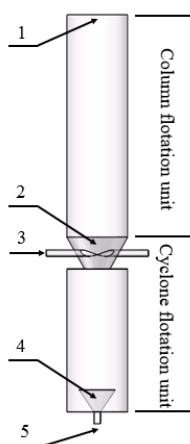
Fig. 4. Schematic diagram of open FCSMC: 1 - concentrate outlet, 2 - cyclonic reversal cone, 3 - middlings inlet, 4 - upright cone, 5 - middlings outlet
