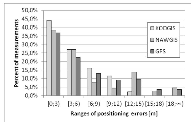
Figure 4. Comparison of DGPS based KODGIS, NAWGIS and embedded GPS receiver positioning accuracy.
