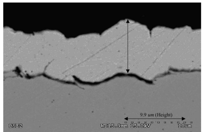
Fig. 14. Copper deposition distributed across each line after 20 scans with different scanning speeds: a) 100 mm/s, b) 200 mm/s, c) 300 mm/s, with the laser power of 3.3 W; SEM micrograph cross-section of the copper track illustrating the copper plating in the electrode–electrolyte interface (b), Ref. 31
