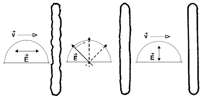
Fig. 6. Results of cutting with parallel, circular and perpendicular polarized laser beam after Ref. 27
