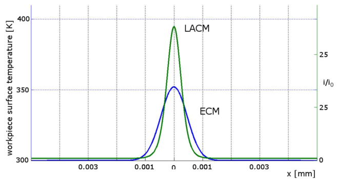
Fig. 11. The effect of workpiece surface temperature increase on current increase, \Delta T = 60 K, w_o = 1.8 mm
