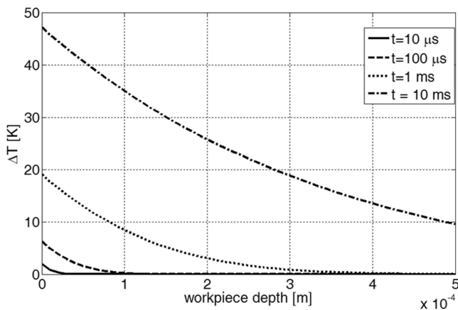
Fig. 10. Temperature rise in material depending on processing time for v = 10 mm/min and laser beam w_o = 1.8 mm
