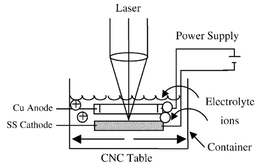
Fig. 13. Laser-controlled selectively electroplating configuration, Ref. 31
