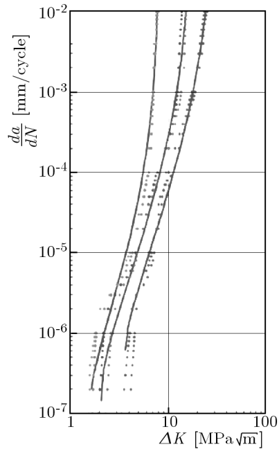
Fig. 5. Approximation of da/dN - \Delta K test data based on modified LSM criterion (3.1)
