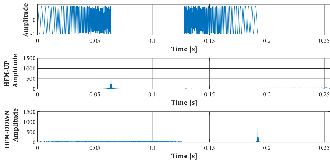
Fig. 3. The frame preamble signal and the determined correlation functions for the received signal with the pattern HFM-UP and HFM-DOWN signals ( T_{sp}=64 ms, T_c=64 ms).
