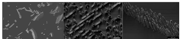
Fig. 3. The various morphologies of the Zn_{16}Ti intermetallic phase [7]
