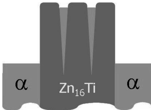
Fig. 5. Model of the block macro-particle
