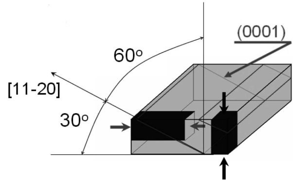
Fig. 2. Primary single crystal and cut off method of samples for the compression test
