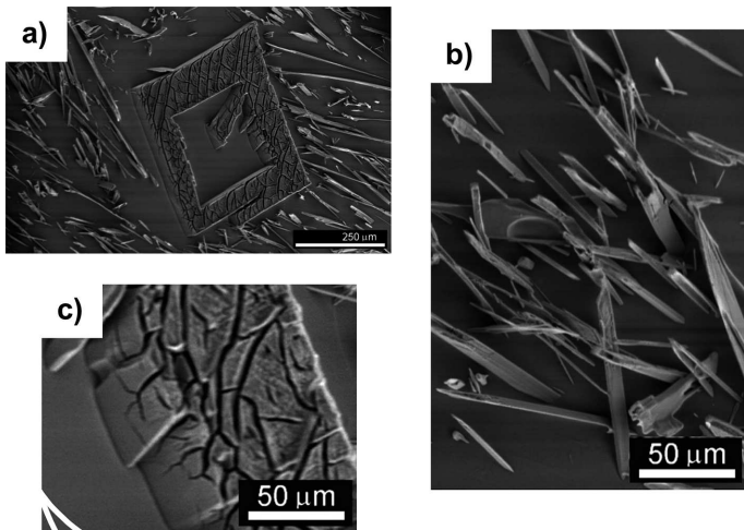
Fig. 4. The block macro-particle (c) and needle-shaped forms (b) of the Zn_{16}Ti phase
