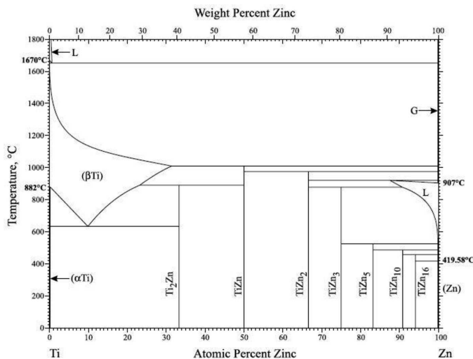
Fig. 1. Zn-Ti phase diagram, Okamoto 2008 [8]
