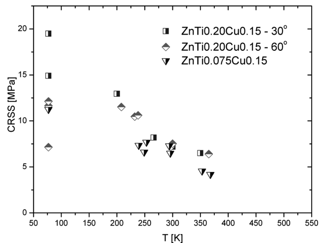
Fig. 7. The CRSS relation to the temperature for two variants of samples orientation. For compare were presented results for Zn-Ti0.075-Cu0.15 single crystals. The anomaly zone was existed only for single crystals with smaller content of titanium
