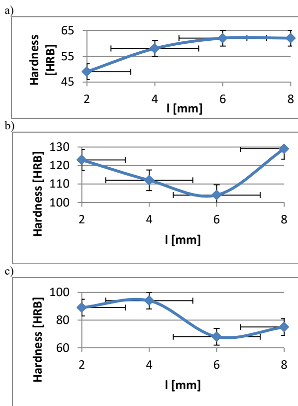
Fig. 4. a) MO59 brass – chill – mold, b) MO59 brass – shell mold, c) M95 brass – shell mold. For each graph were added the so-called error bars using a standard error
