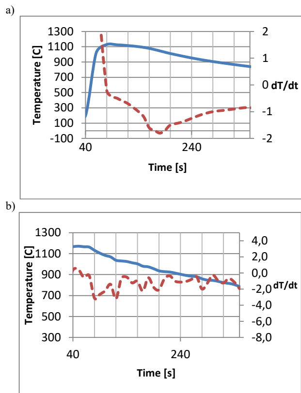
Fig. 3. M95 brass cooling curves a) temperature course [ ^{\circ}\text{C} ] over time, b) cooling curve of the liquid alloy free surface - pyrometer measurement (dotted line)
