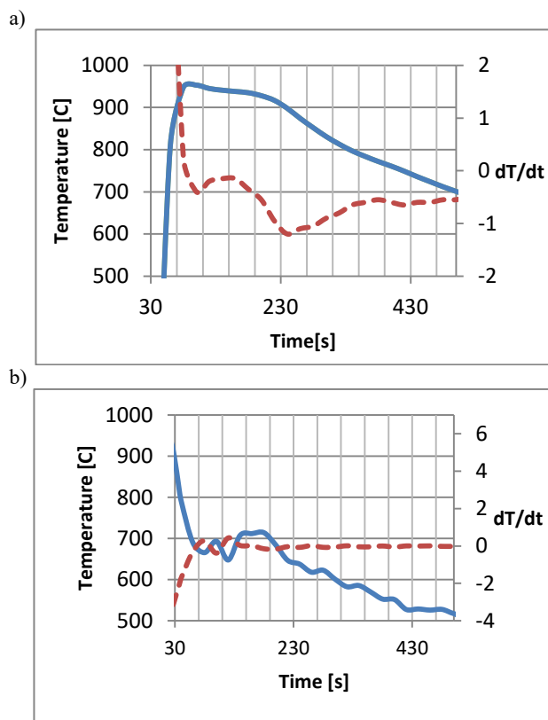
Fig. 2. MO59 brass cooling curves a) temperature course [ ^{\circ}\text{C} ] over time, b) cooling curve of the liquid alloy free surface - pyrometer measurement (dotted line)
