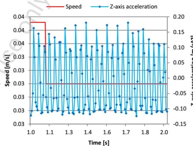
Fig. 6. Z-axis values and speed recorded while the user is running and the phone is placed in the jacket pocket
