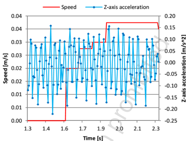
Fig. 5. Z-axis values and speed recorded while the user is running and the phone is placed in the trousers pocket
