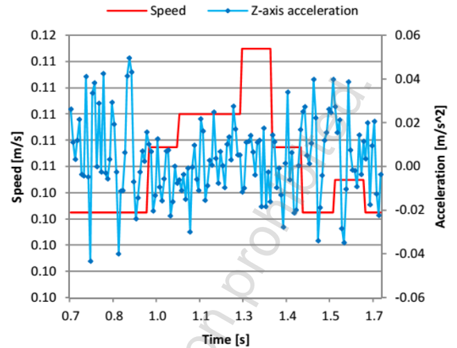
Fig. 8. Z-axis values and speed recorded while driving car#1 on an uneven road and the smartphone is placed horizontally on the dashboard
