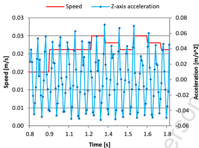
Fig. 4. Z-axis values and speed recorded while the user is walking and the phone is placed in the jacket pocket
