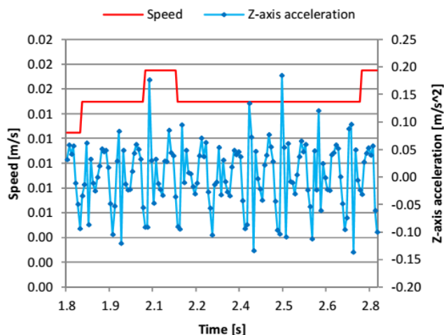
Fig. 3. Z-axis values and speed recorded while the user is walking and the phone is placed in the trousers pocket
