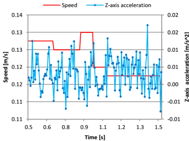
Fig. 9. Z-axis values and speed recorded while driving car#2 on a smooth road and the smartphone is placed horizontally on the dashboard
