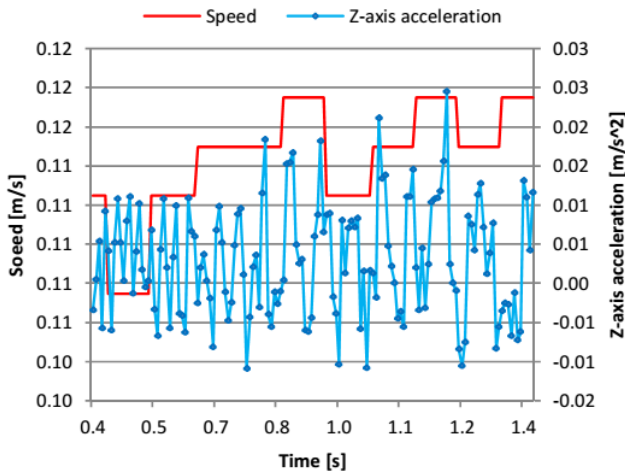
Fig. 7. Z-axis values and speed recorded while driving car#1 on a smooth road and the smartphone is placed horizontally on the dashboard
