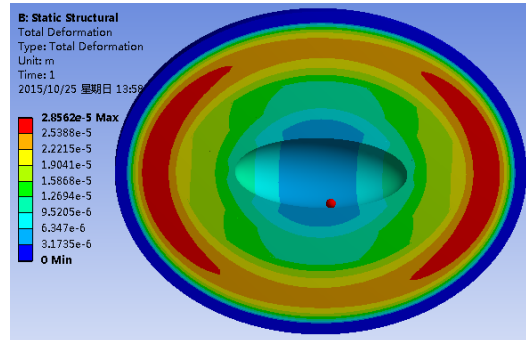
Figure 20: The total deformation contour of ellipsoid.
