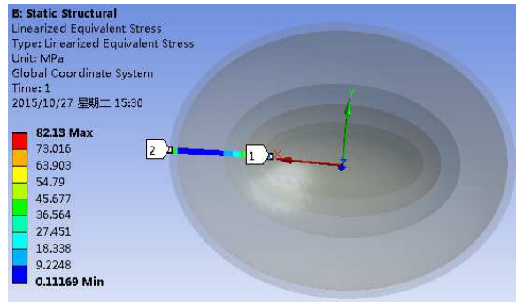
Figure 27: Radial linear stress.
