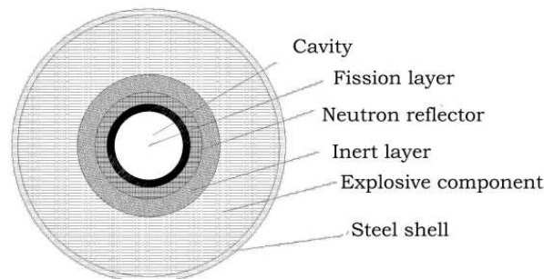
Figure 1: Schematic diagram of complicated multiplelayer components.
