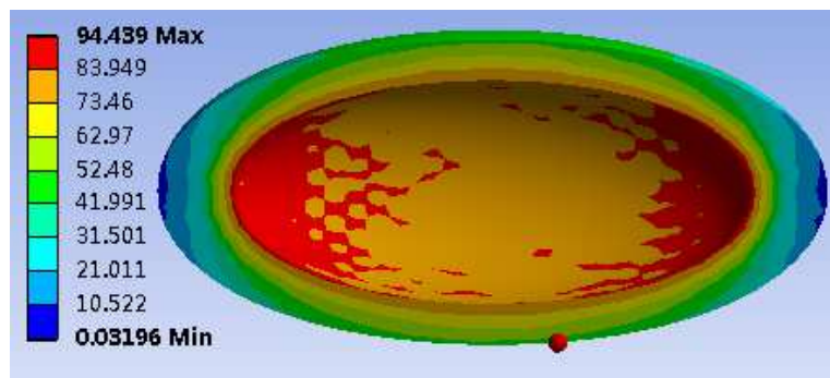
Figure 24: Stress contour of beryllium part.
