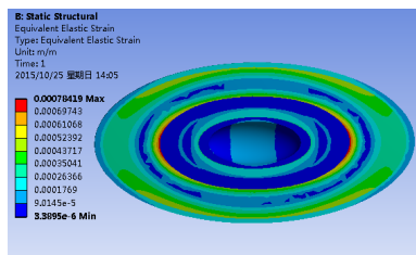
Figure 22: Equivalent elastic strain diagram.
