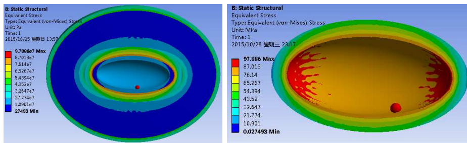
Figure 16: Equivalent elastic strain. Figure 17: Equivalent strain contour of explosive.
