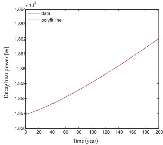
Figure 3: Plutonium decay power.
