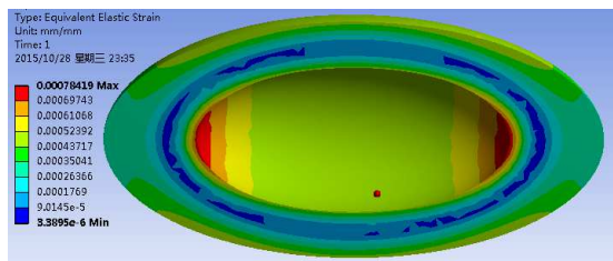
Figure 23: Elastic strain diagram of explosive parts.
