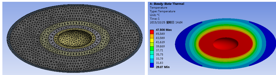
Figure 21: Grid division and temperature stress contour of ellipsoid.
