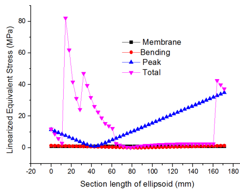
Figure 26: Four kinds of radial linear stress.
