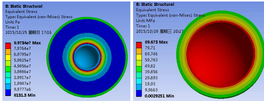
Figure 10: Equivalent stress contour. Figure 11: Equivalent stress contour of beryllium.
