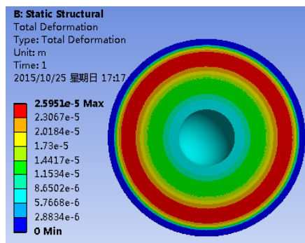
Figure 12: Total deformation contour of sphere structure.
