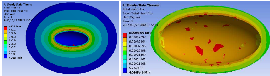
Figure 14: Heat flow density contour. Figure 15: Heat flow density contour of beryllium.
