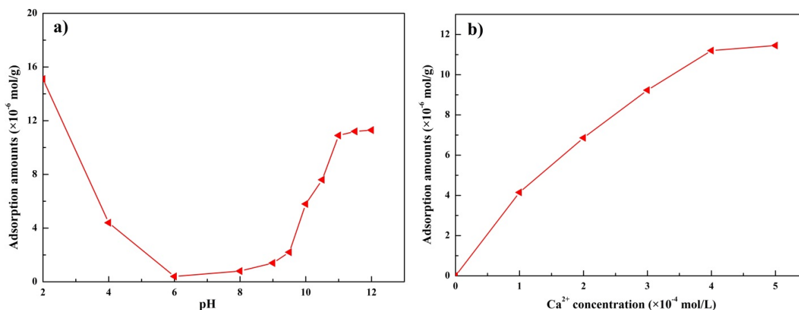
Fig. 3. Adsorption amounts of sodium oleate on quartz surfaces (a) as a function of pH and (b) \text{Ca}^{2+} concentration
