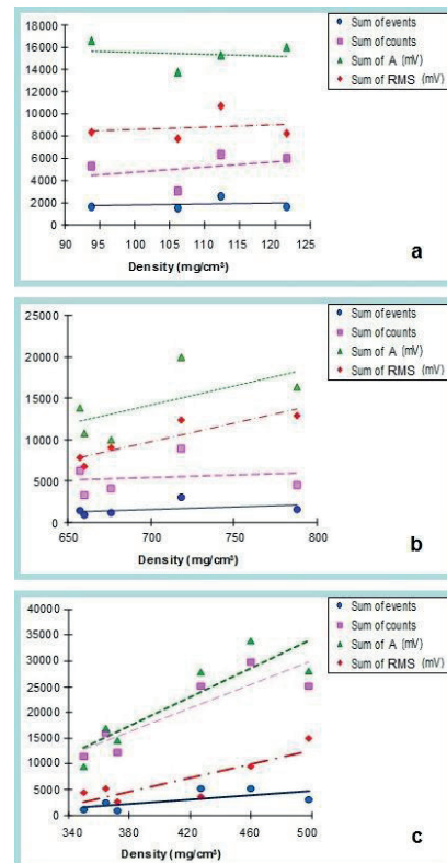
Fig. 7. Evolution of four AE parameters depending on densities of composites. a) CEG, b) POL, c) CARB
