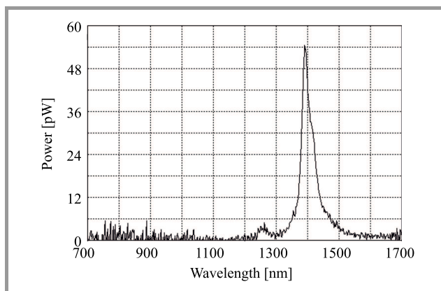
Fig. 17. Spectrum of thermal emission for the OFS MM50 fiber at 900°C in test 1.
