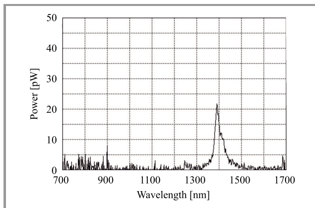
Fig. 16. Spectrum of thermal emission for the OFS MM50 fiber at 800°C in test 1.
