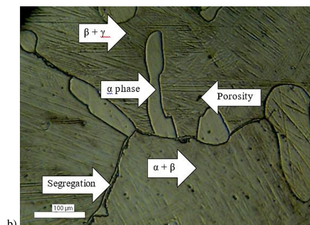
Figure 6. The microstructure (a) Sand Casting Non-Treatment/SCNT (b) Sand Casting Heat Treatment/SCHT
