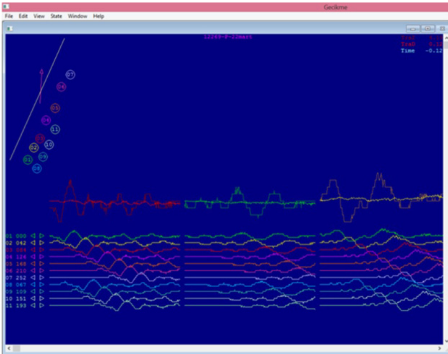
Fig. 14. The group-blast-induced seismic waves screen. The time-delays are at 42 ms between the blast-holes and 67 ms between blast-lines
