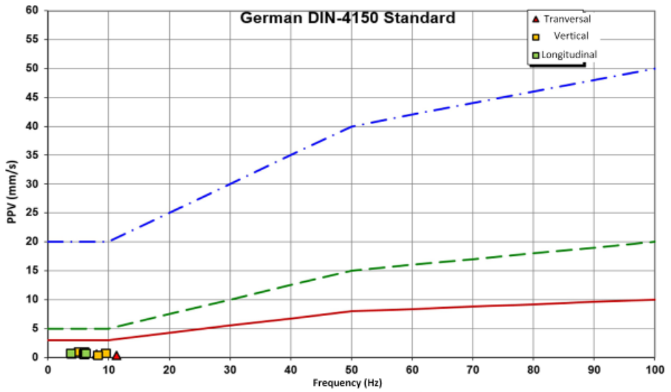
Fig. 12. German DIN-4150 Standard
