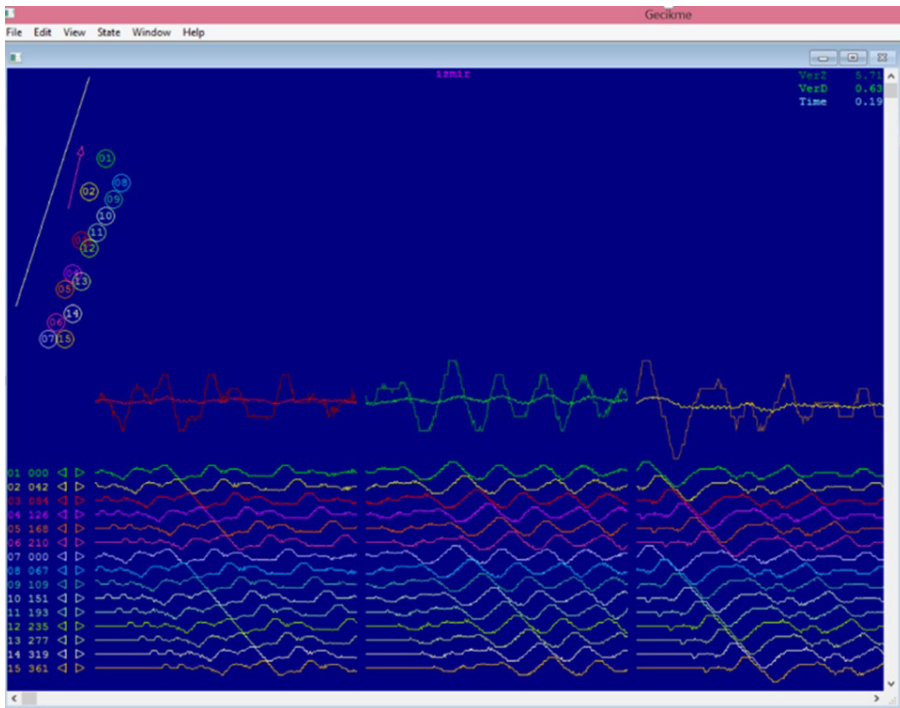
Fig. 7. Model for delays at 42 ms between blast-holes and 67 ms surface delay
