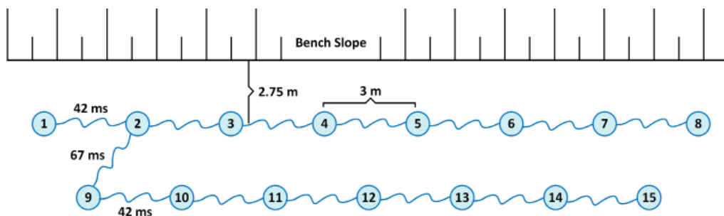
Fig. 6. The blast-hole design with 15 holes
