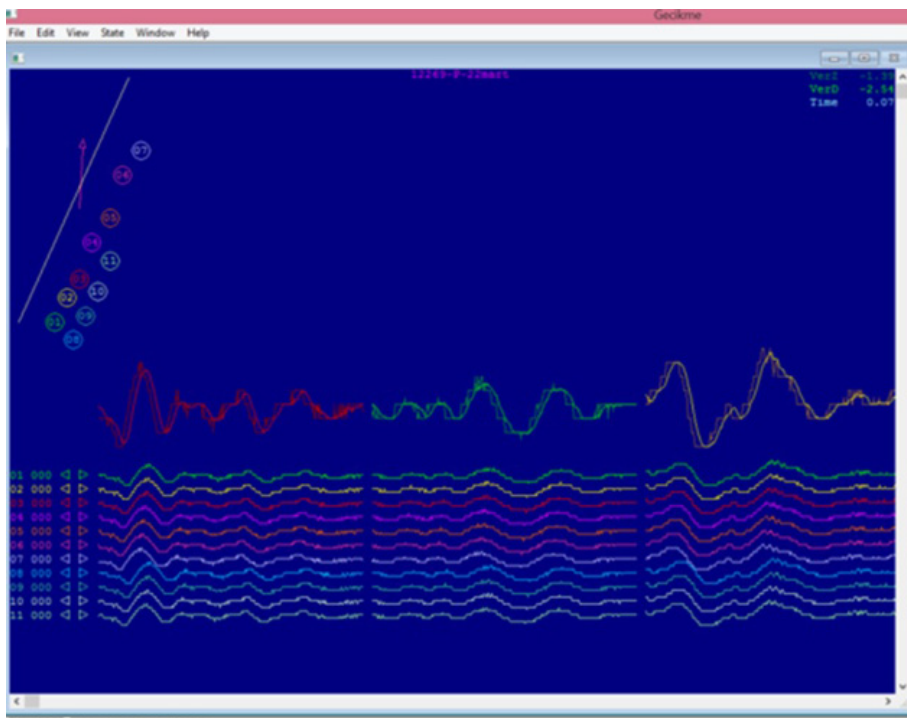
Fig. 13. The pilot-blast-induced seismic waves screen. There are no time-delays yet
