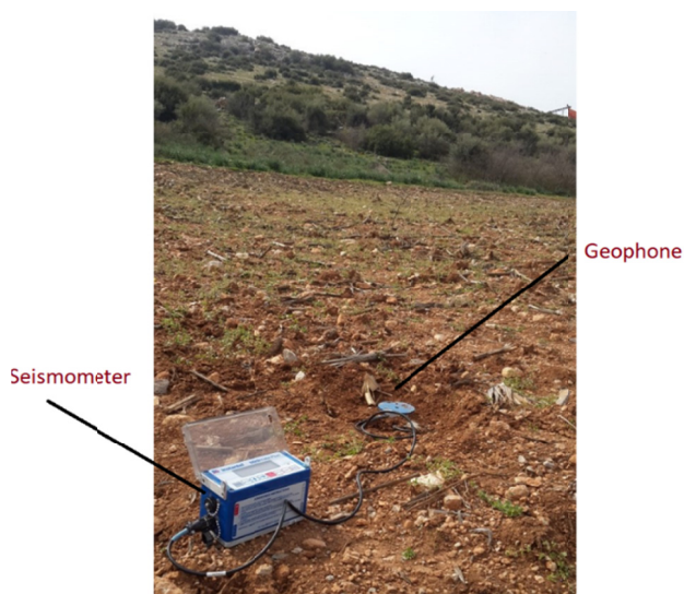
Fig. 2. Seismometer and geophone
