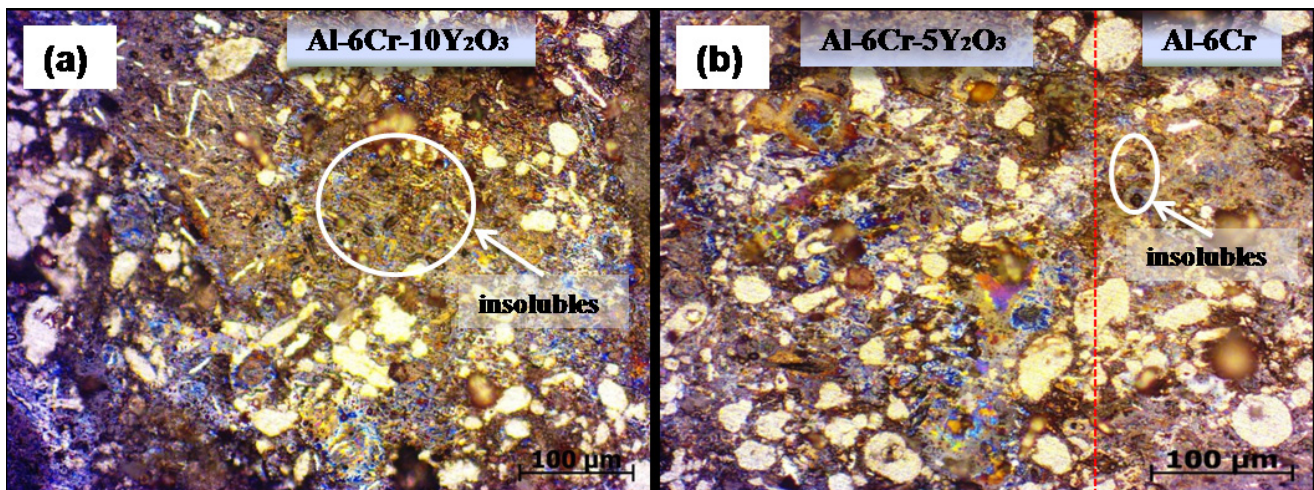
Fig. 3. Polarized light micrograph shows different regions of FGM Al-6Cr alloy a) Al-6Cr-10 Y_2O_3 , b) Al-6Cr-5 Y_2O_3 and Al-6 vol% Cr alloy in age hardened condition
