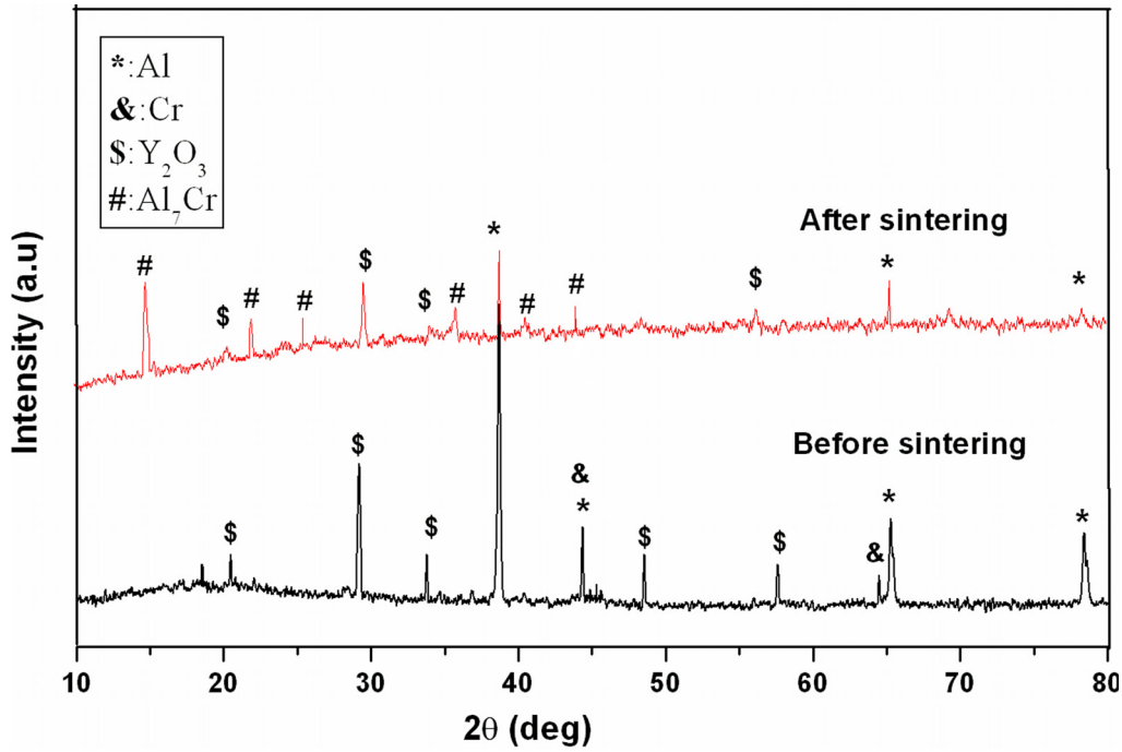
Fig. 5. X-ray diffraction patterns for all the composites
