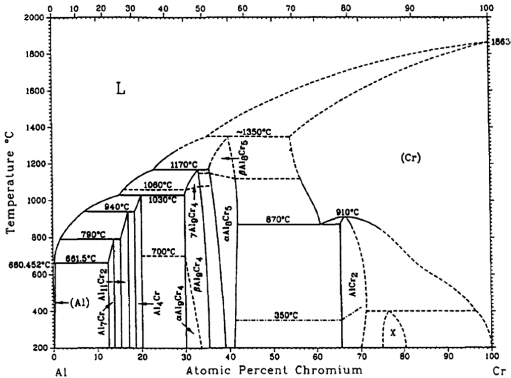
Fig. 6. Al-Cr phase diagram (from Okamoto [22])
