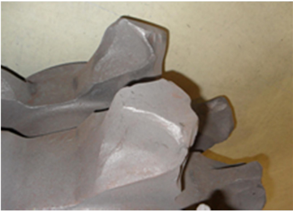
Fig. 1. An example view of tribocorrosive wear of a chain wheel in an armoured face conveyor
