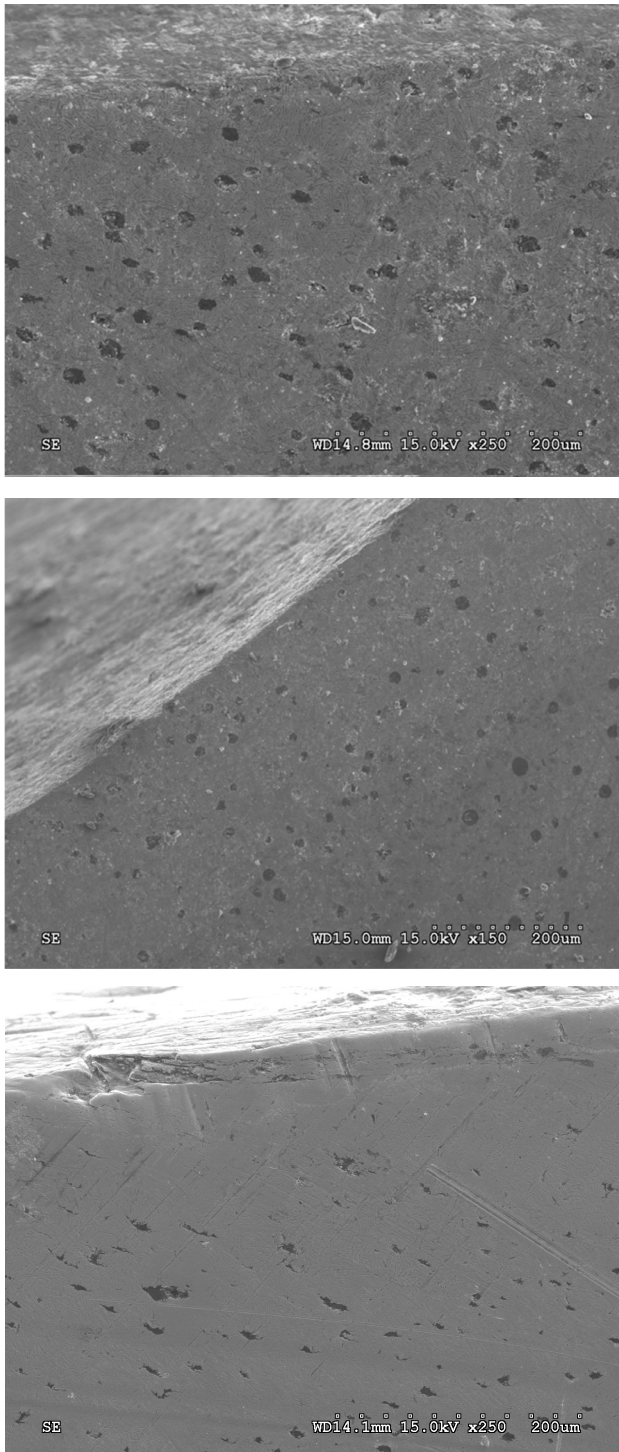
Fig. 13. The microstructure in an area of 0 \div 1 mm under the surface subject to wear in abrasive conditions; lower figure show microstructure of ADI_360, medium figure and upper figure shows microstructure of ADI_360_COR
