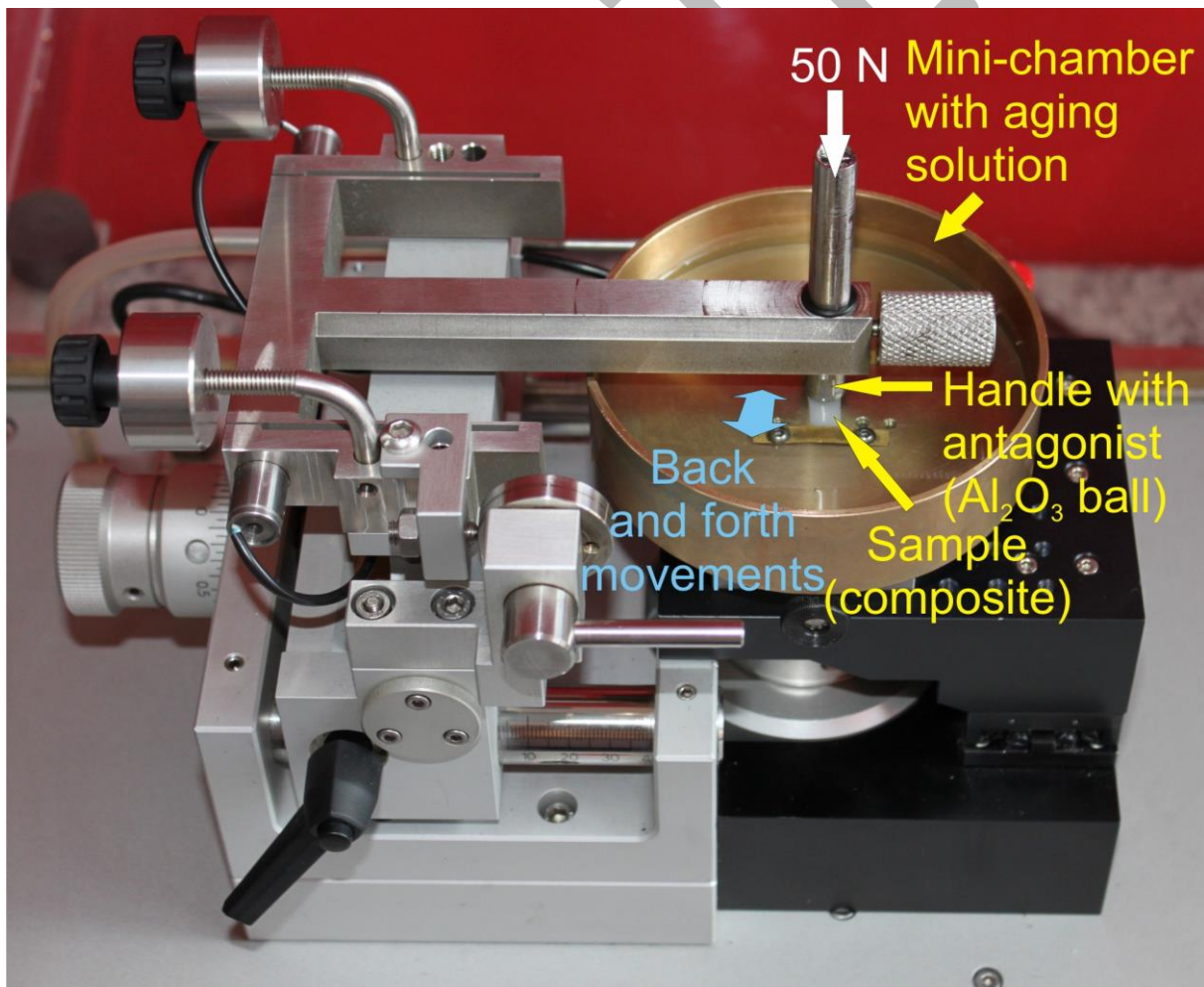
Fig. 1. Tribometer with the environmental mini-chamber attached.
