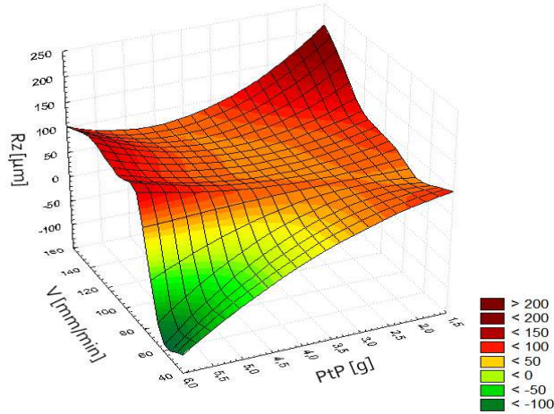
Fig. 9. Dependence of the surface roughness parameter Rz on the average of absolute values of material vibrations Peak-to-Peak and the traverse speed of cutting head v appertaining to (5).
