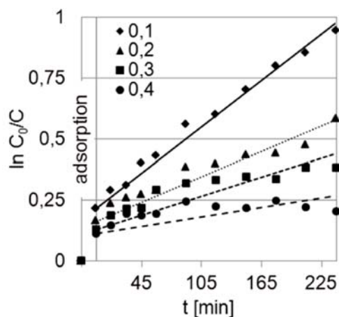
Figure 8. Kinetics of the degradation of sertraline in the flow reactor for different initial concentrations [g/dm 3 ] of sertraline in the supported system
