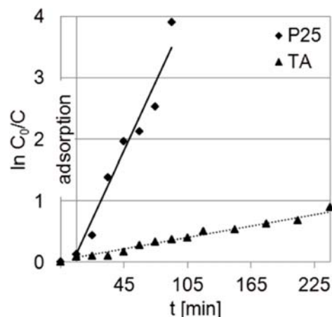
Figure 10. Comparison of the photocatalytic activity of TA and P25 materials. Initial concentration of sertraline – 0.025 g/dm 3 , amount of photocatalyst – 1.15 g/dm 3
