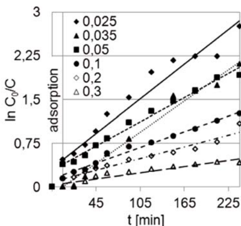
Figure 6. Kinetics of the photocatalytic degradation of sertraline in the periodic reactor for different initial concentrations [\text{g/dm}^3] of sertraline in the supported system
