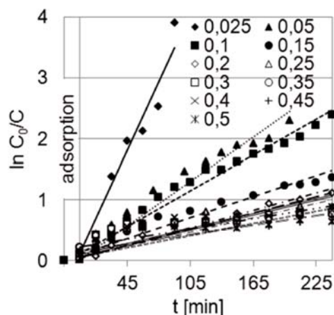
Figure 5. Kinetics of the photocatalytic degradation of sertraline in the periodic reactor for different initial concentrations [\text{g/dm}^3] of sertraline with suspended \text{TiO}_2 . Amount of photocatalyst – 1.15 \text{ g/dm}^3
