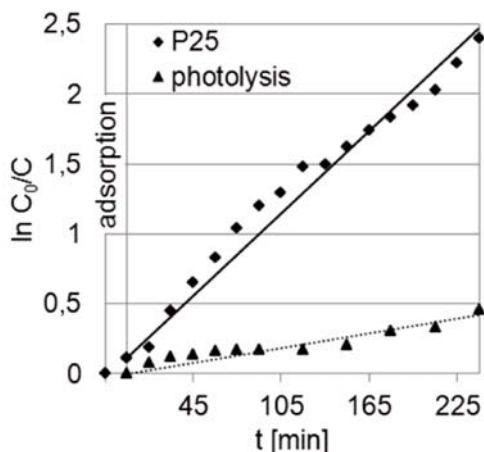
Figure 3. Kinetics of the degradation of sertraline in the periodic reactor by photolysis and photocatalysis using suspended \text{TiO}_2 . Initial concentration of sertraline – 0.1 \text{ g/dm}^3 , amount of photocatalyst – 1.15 \text{ g/dm}^3
