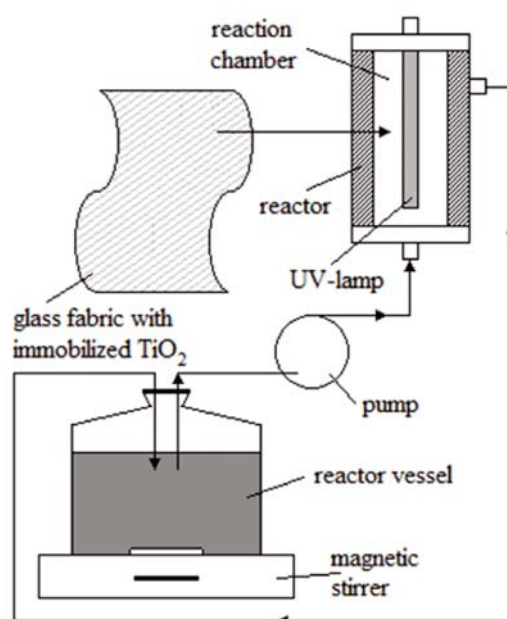
Figure 2. Scheme of the flow photoreactor
