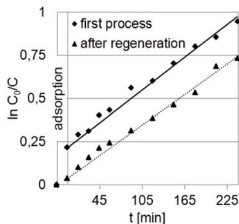
Figure 9. Comparison of the photocatalytic degradation of sertraline with application of fresh and regenerated glass fabric. Initial concentration of sertraline – 0.1 g/dm 3
