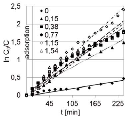
Figure 4. Kinetics of the photocatalytic degradation of sertraline in the periodic reactor for different amount [\text{g/dm}^3] of suspended \text{TiO}_2 . Initial concentration of sertraline – 0.1 \text{ g/dm}^3
