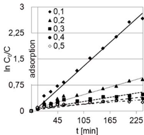
Figure 7. Kinetics of the photocatalytic degradation of sertraline in the flow reactor for different initial concentrations [g/dm 3 ] of sertraline with suspended TiO 2 . Amount of photocatalyst – 0.5 g/dm 3
