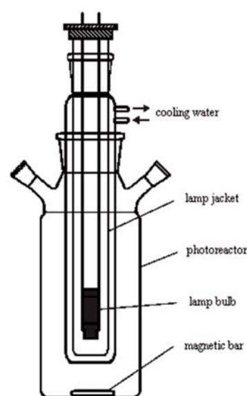
Figure 1. Scheme of the batch photoreactor with a medium pressure mercury lamp
