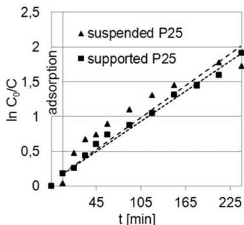
Figure 11. Comparison of the photocatalytic activity of suspended and supported P25. Initial concentration of sertraline – 0.1 g/dm 3 , amount of photocatalyst – 0.25 g per reaction volume
