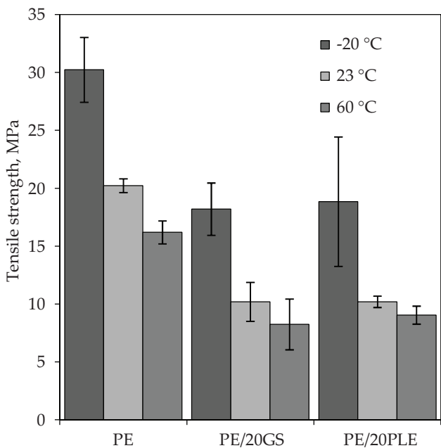
Fig. 6. Comparison of tensile strength for the neat PE and its blends with 20 wt % of biopolymers at different temperatures
