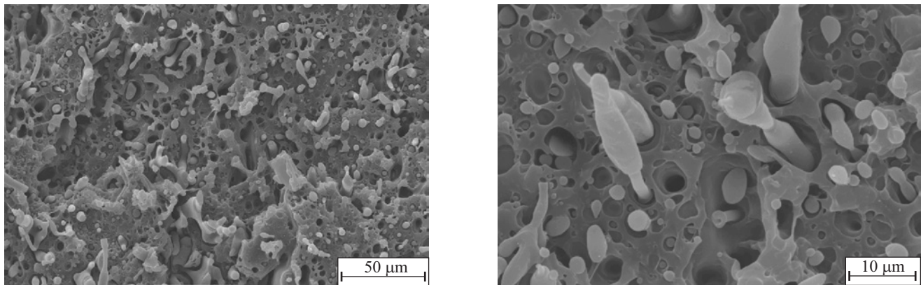
Fig. 2. Low- and high-magnification SEM images of PE/20PLE tensile test fracture surfaces
