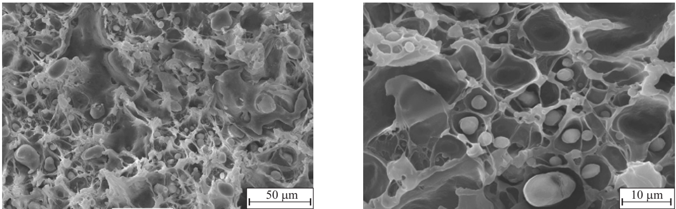
Fig. 1. Low- and high-magnification SEM images of PE/20GS tensile test fracture surfaces
