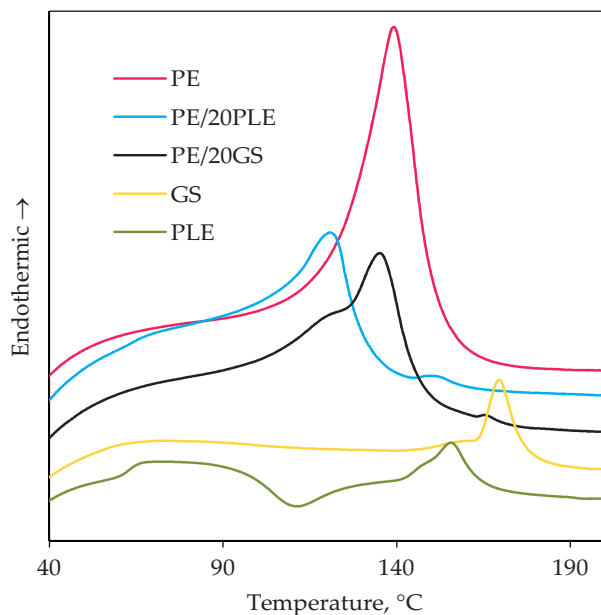
Fig. 8. DSC heating curves for neat PE, biopolymers and for PE blends with 20 wt % of biopolymers in the second heating-cooling cycle
