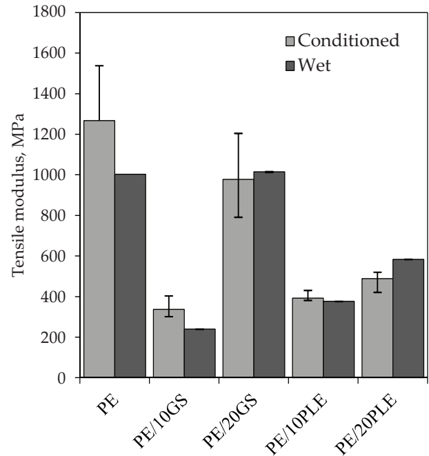
Fig. 5. Tensile modulus of the conditioned materials and after 14 days of soaking
