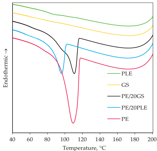
Fig. 9. DSC cooling curves for neat PE, biopolymers and for PE blends with 20 wt % of biopolymers in the second heating-cooling cycle
