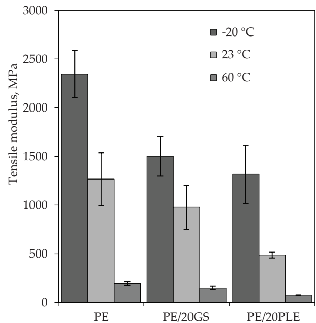
Fig. 7. Comparison of tensile modulus for the neat PE and its blends with 20 wt % of biopolymers at different temperatures
