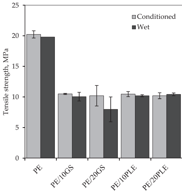
Fig. 4. Tensile strength of the conditioned materials and after 14 days of soaking
