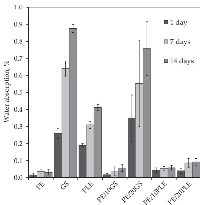
Fig. 3. Water absorption of the tested materials after 1, 7 and 14 days of soaking
