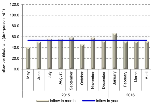
Fig. 6. Inflow of wastewater per inhabitant from house “C”; source: own study
