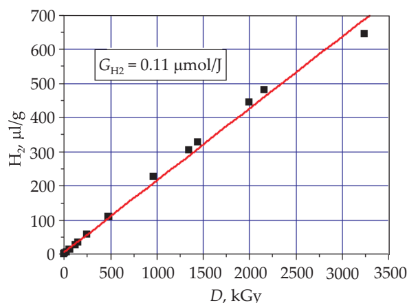
Fig. 4. For the HNBR elastomer, for example, a weld showing the radiolytic efficiency of hydrogen has been shown; in this case, it is an average value for a very large range of radiation doses (up to 3500 kGy)
