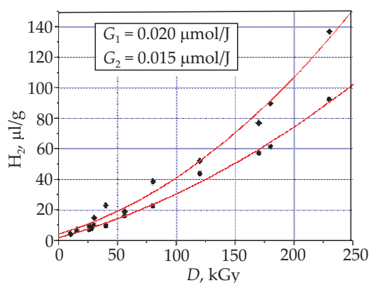
Fig. 5. Radiolytic hydrogen generation curve of two kinds of keratin; hydrogen evolution yields from an exemplary natural polymer, the published yields of G_{H_2} are average in the form of doses up to 250 kGy
