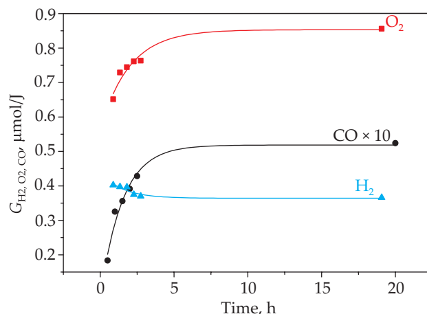
Fig. 2. The phenomenon postradiation degradation of polypropylene; ionizing radiation initiates the process of chain oxidation, the changes in hydrogen, carbon monoxide and oxygen efficiency have been shown as a function of time from irradiation to analysis over time, the yield of carbon monoxide and the efficiency of oxygen absorption by samples of primary polypropylene (without additions of antioxidants and light stabilizers) increases
